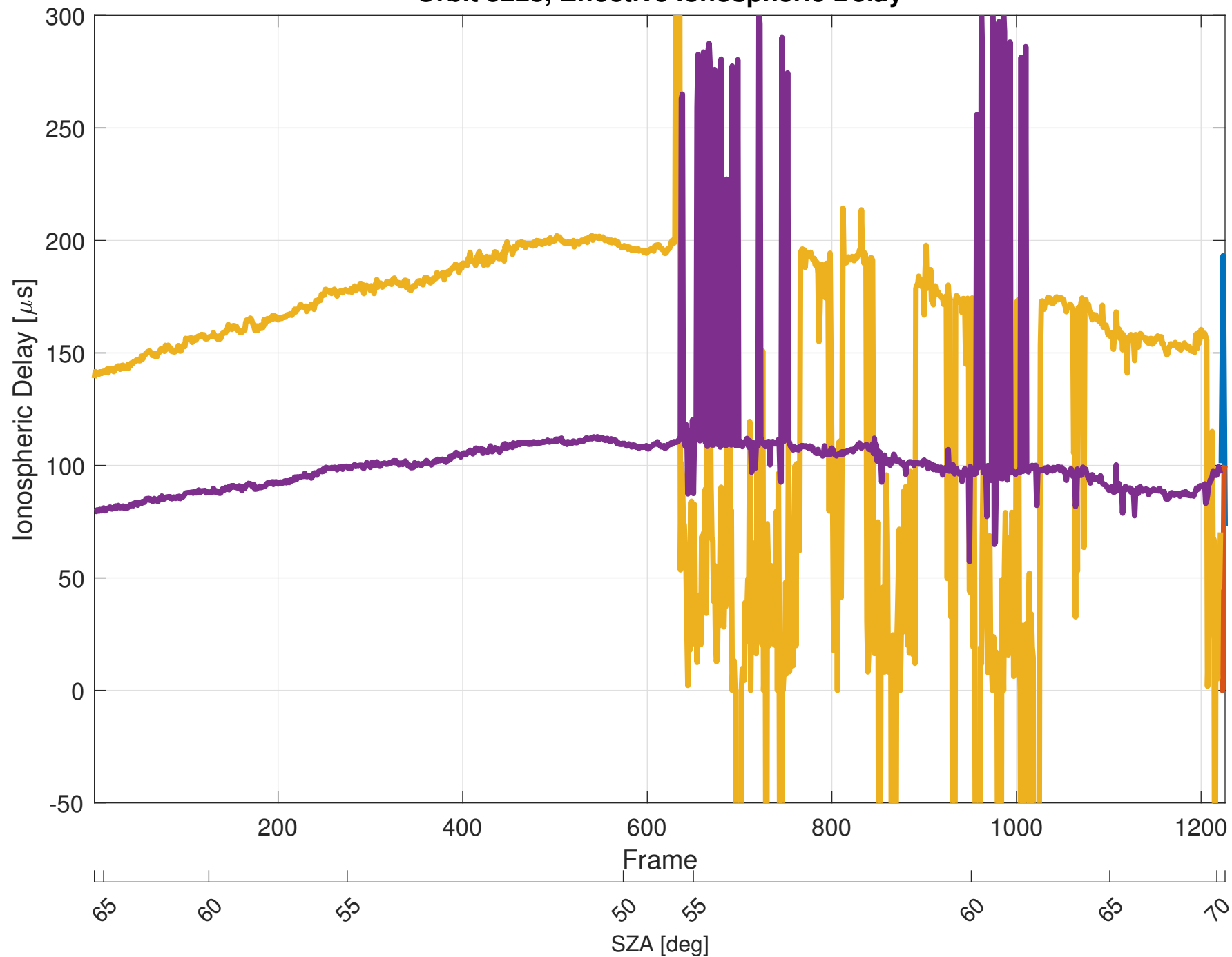
Orbit 5228, Effective Ionospheric Delay
