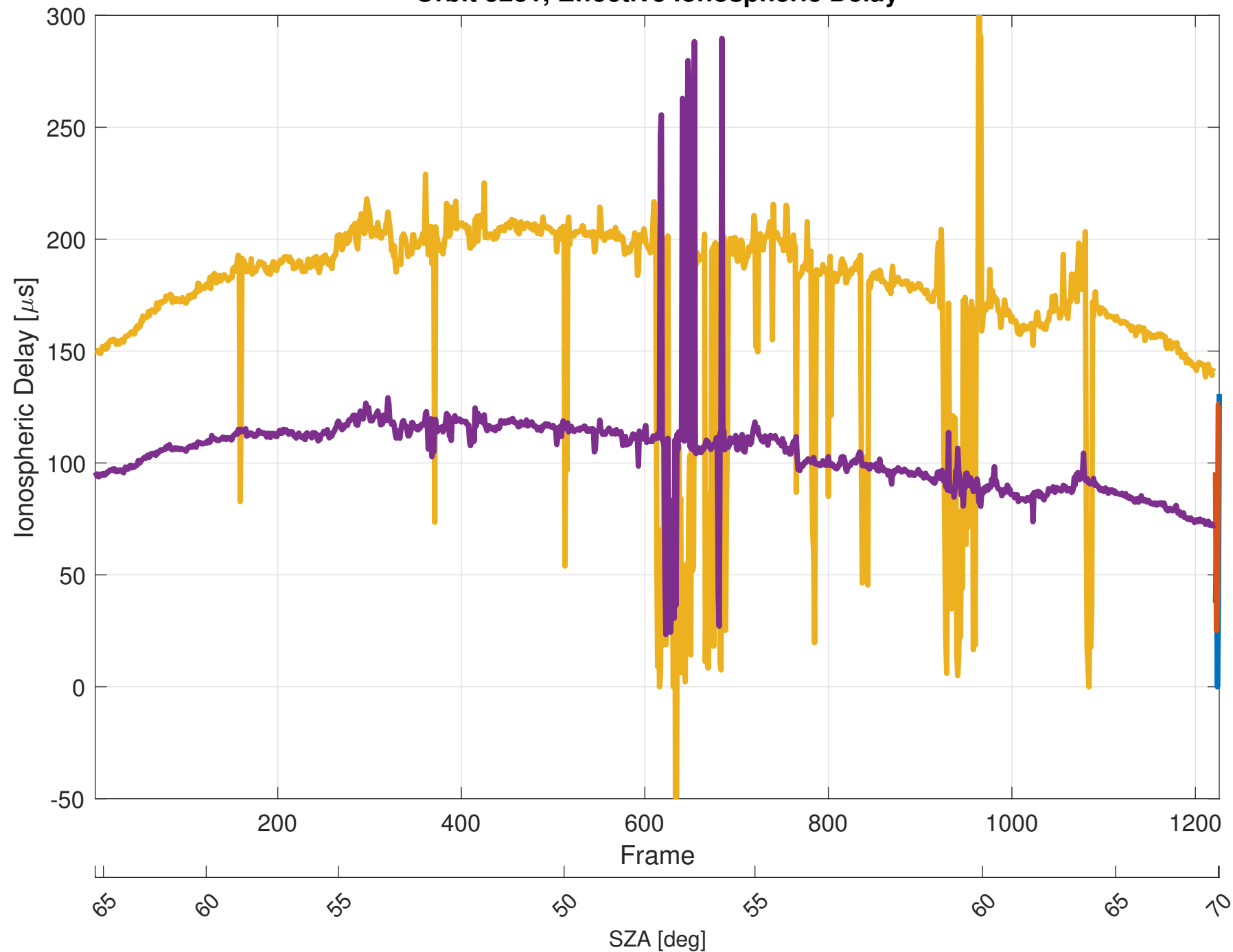
Orbit 5231, Effective Ionospheric Delay
