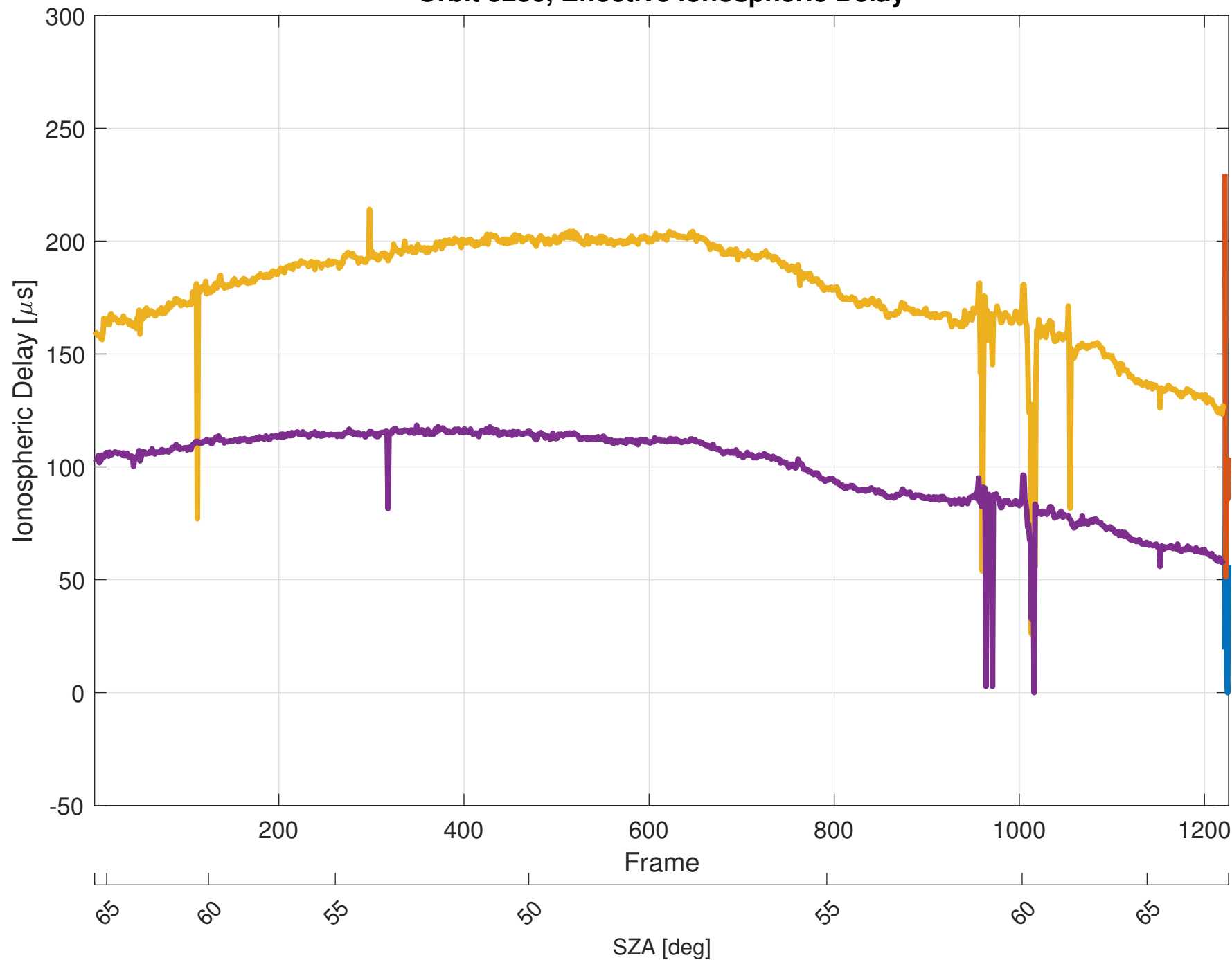
Orbit 5236, Effective Ionospheric Delay
