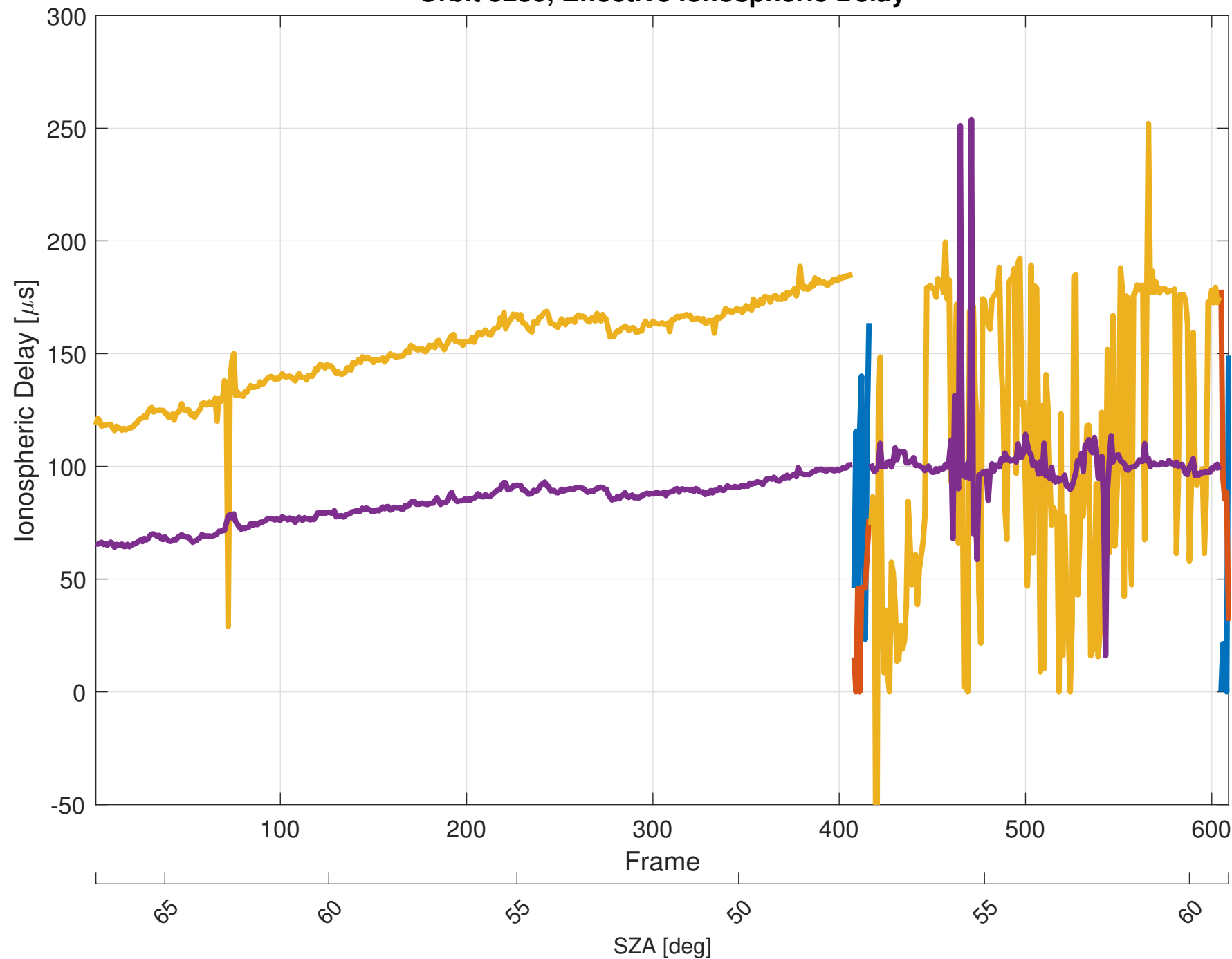
Orbit 5280, Effective Ionospheric Delay
