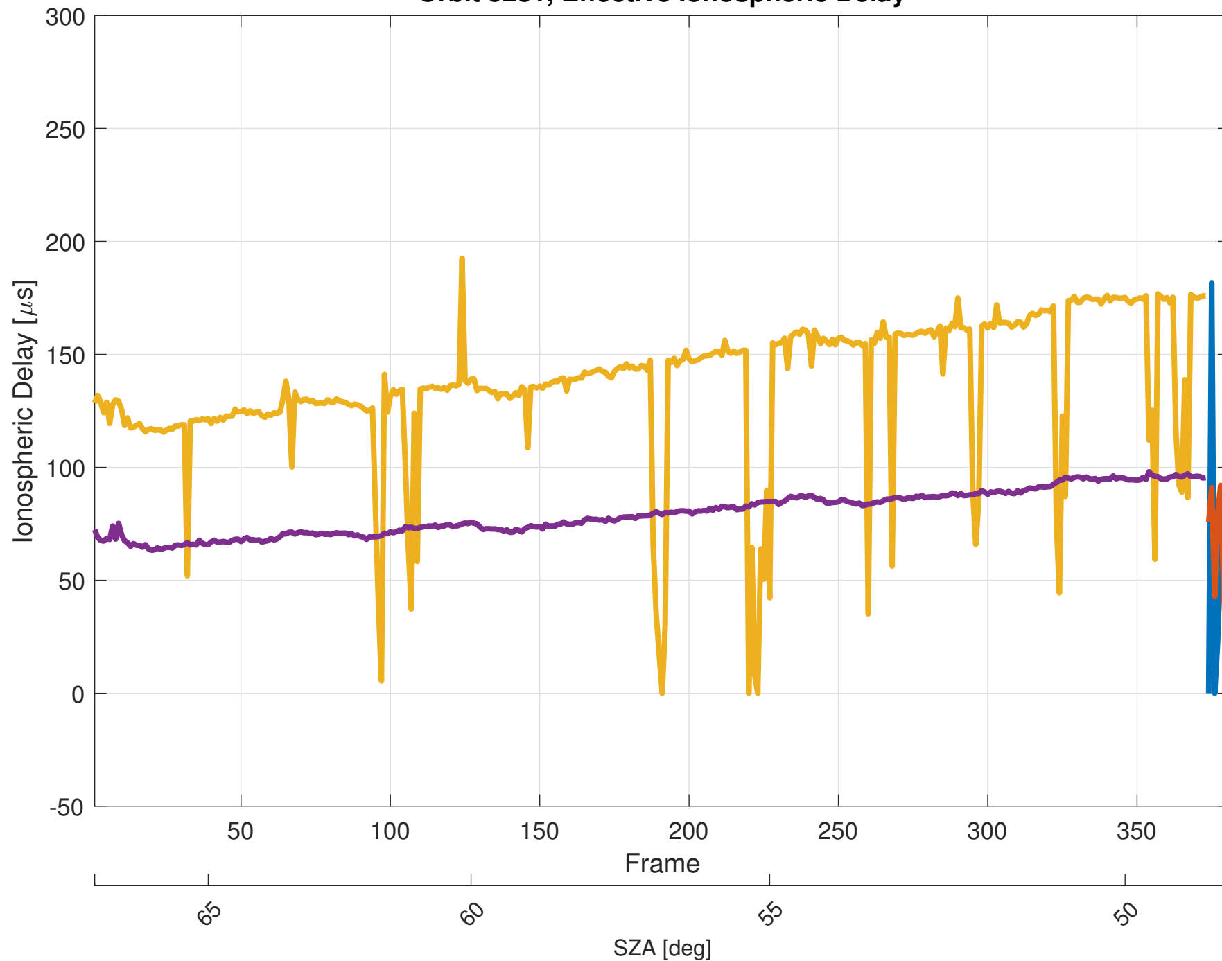
Orbit 5281, Effective Ionospheric Delay
