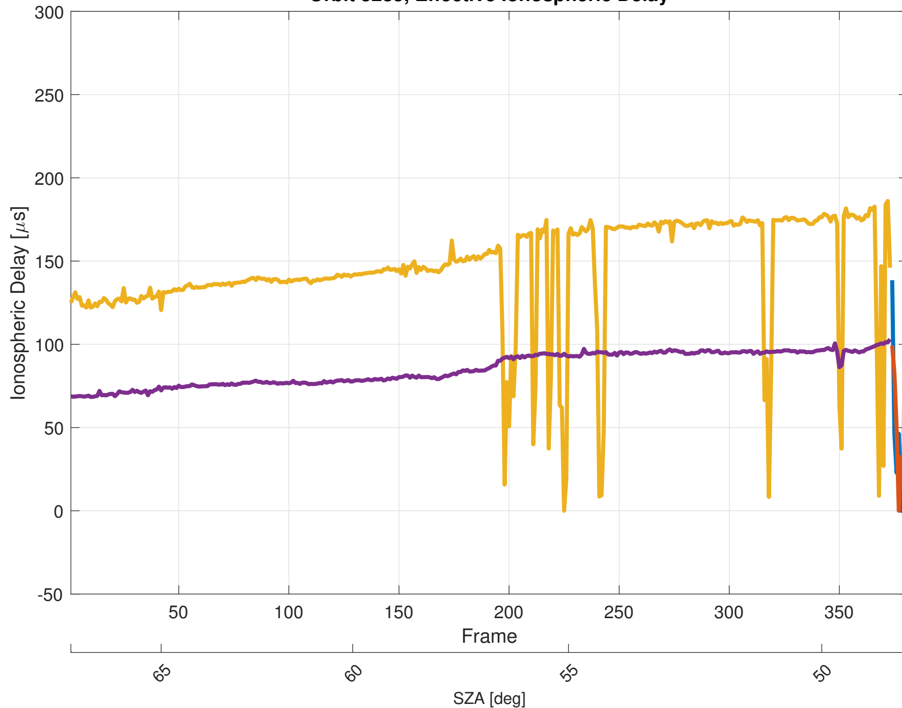
Orbit 5285, Effective Ionospheric Delay
