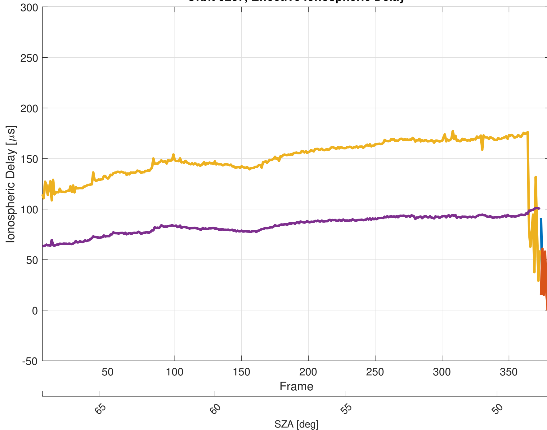
Orbit 5287, Effective Ionospheric Delay
