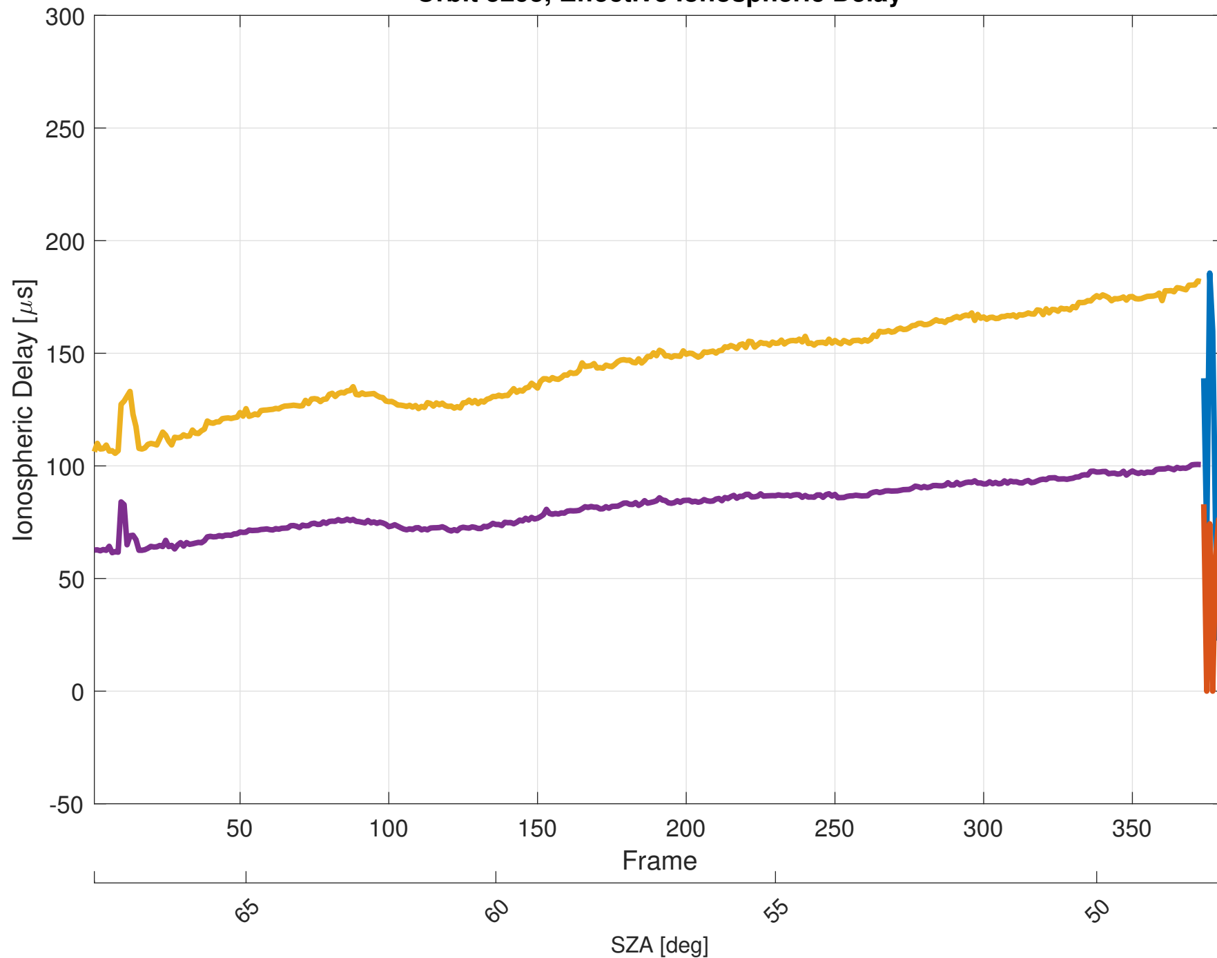
Orbit 5295, Effective Ionospheric Delay
