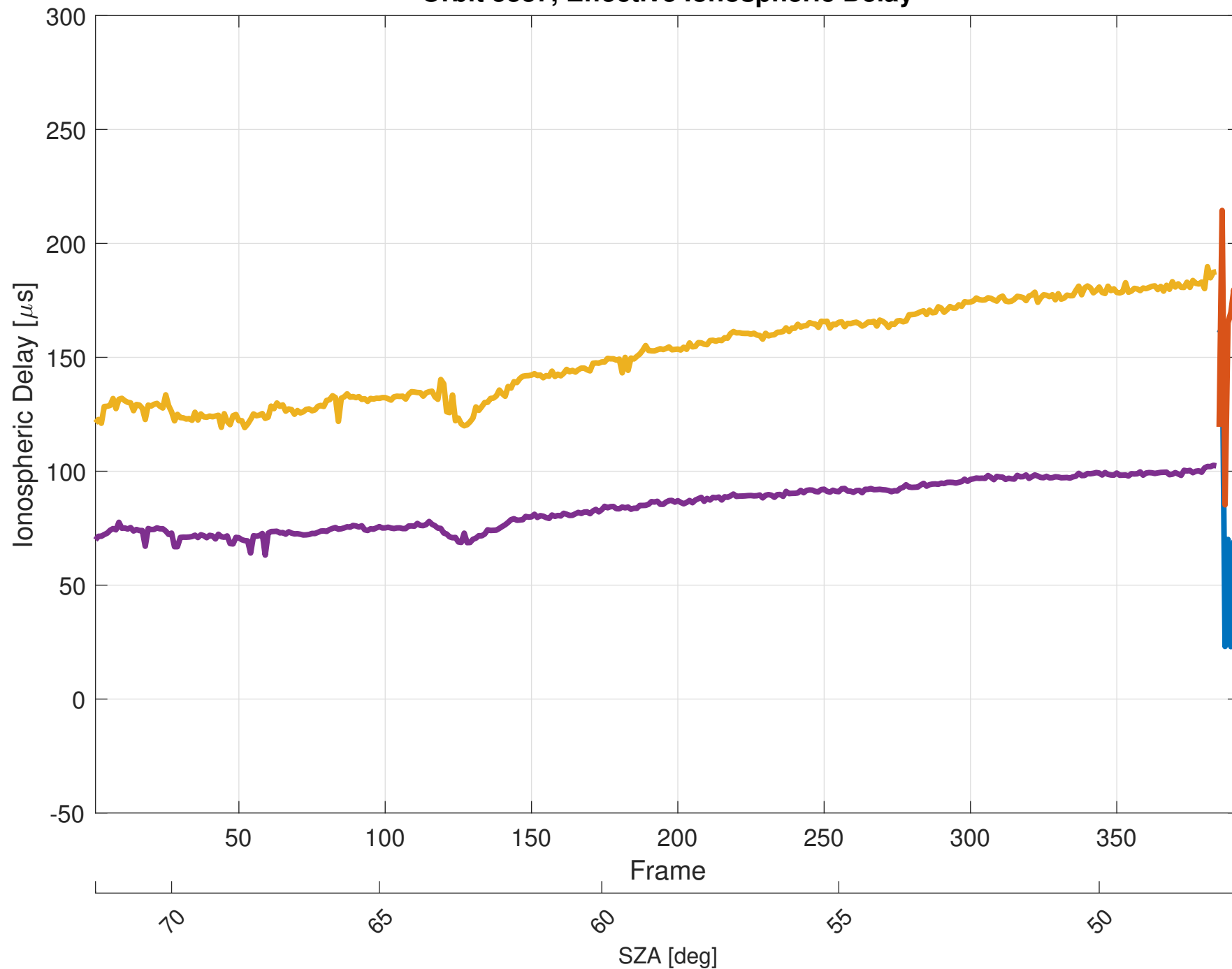
Orbit 5337, Effective Ionospheric Delay
