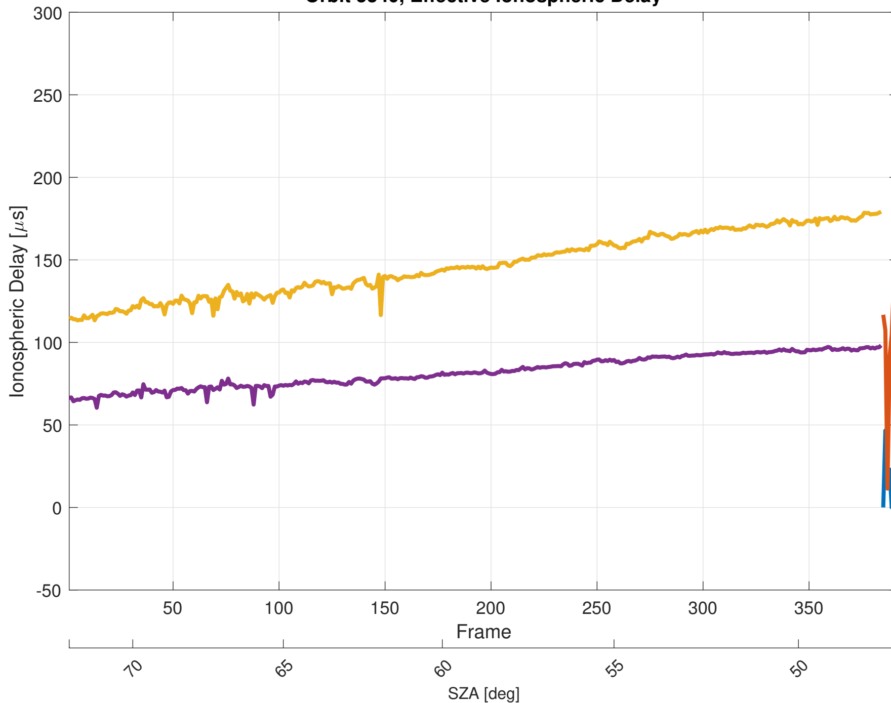
Orbit 5340, Effective Ionospheric Delay
