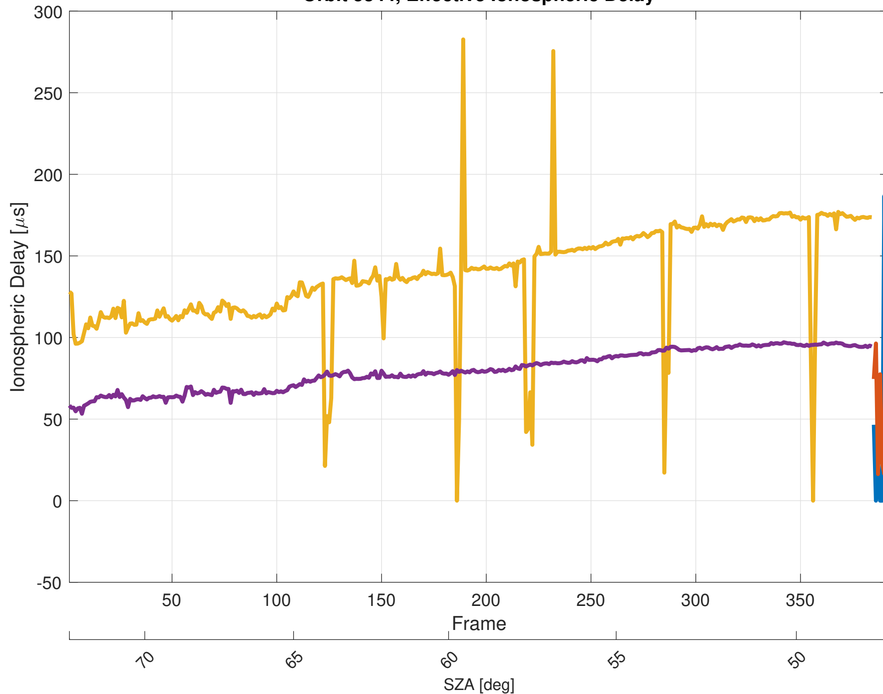
Orbit 5344, Effective Ionospheric Delay
