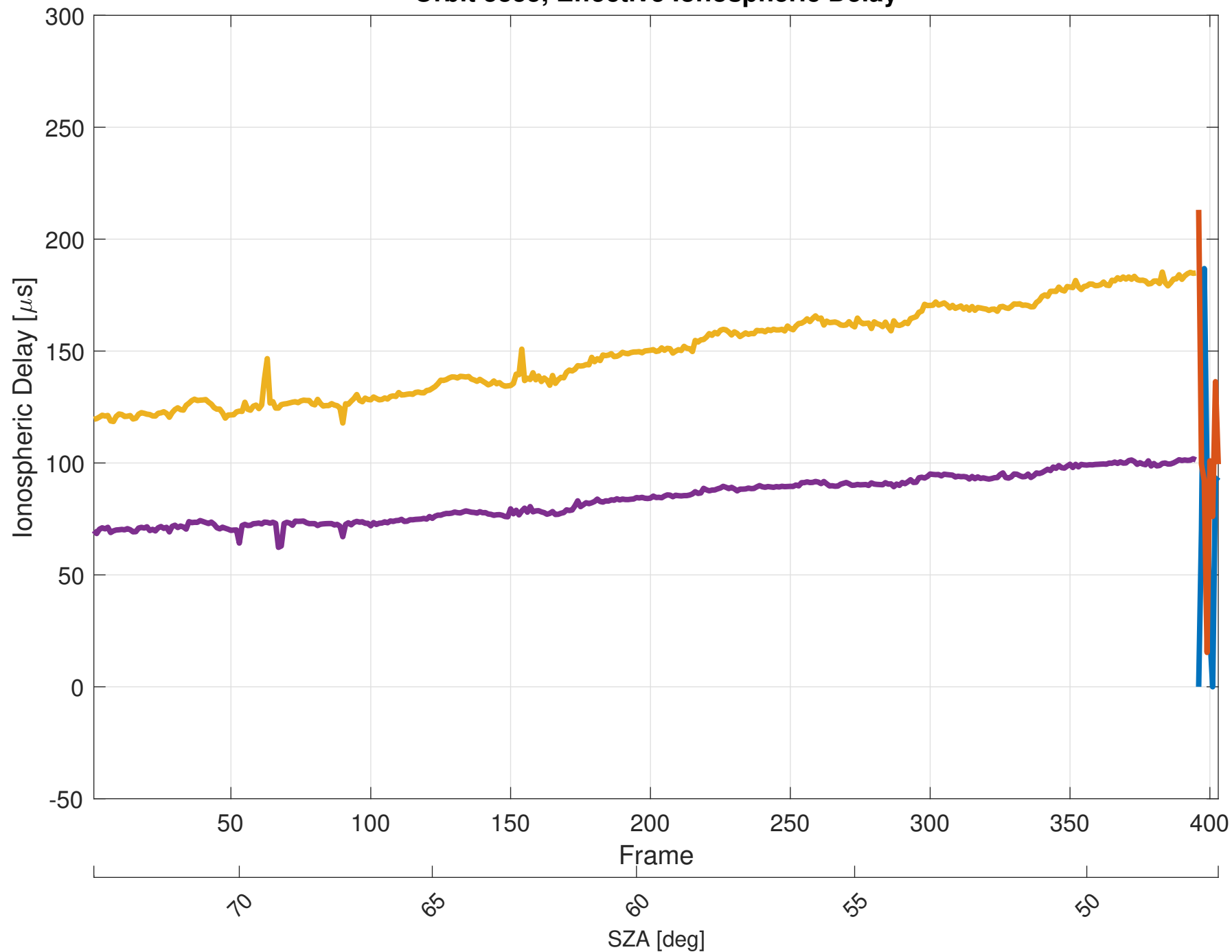
Orbit 5355, Effective Ionospheric Delay
