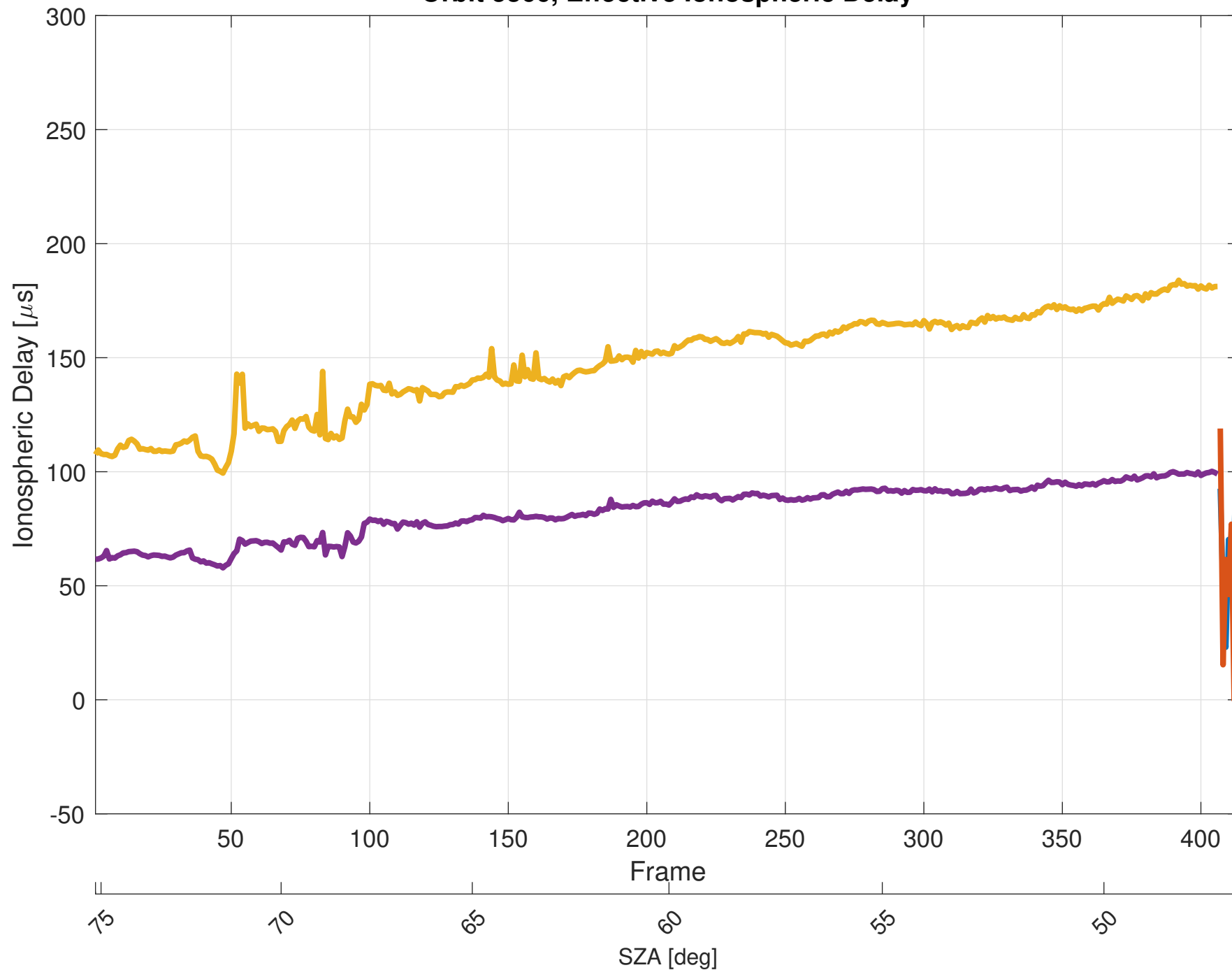
Orbit 5366, Effective Ionospheric Delay
