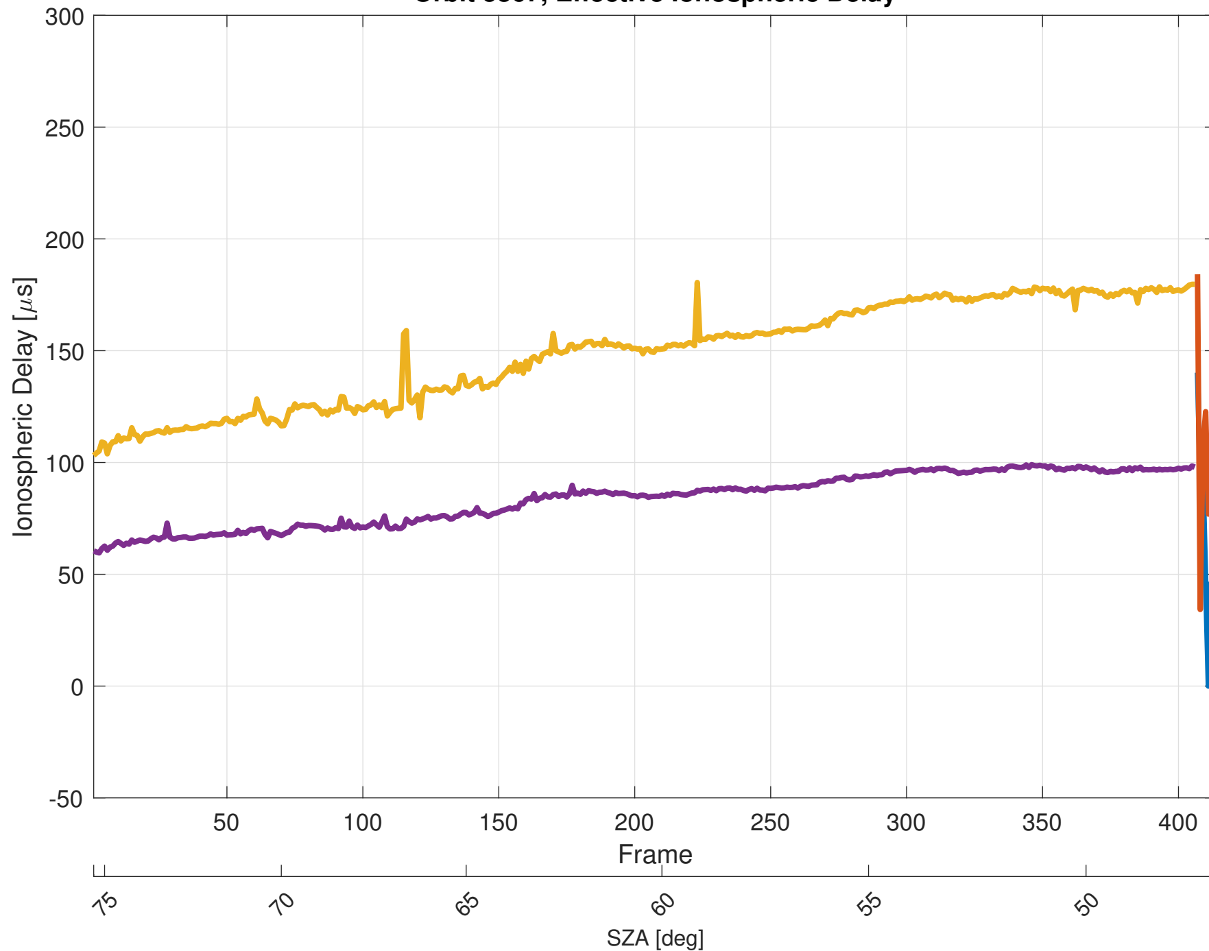
Orbit 5367, Effective Ionospheric Delay
