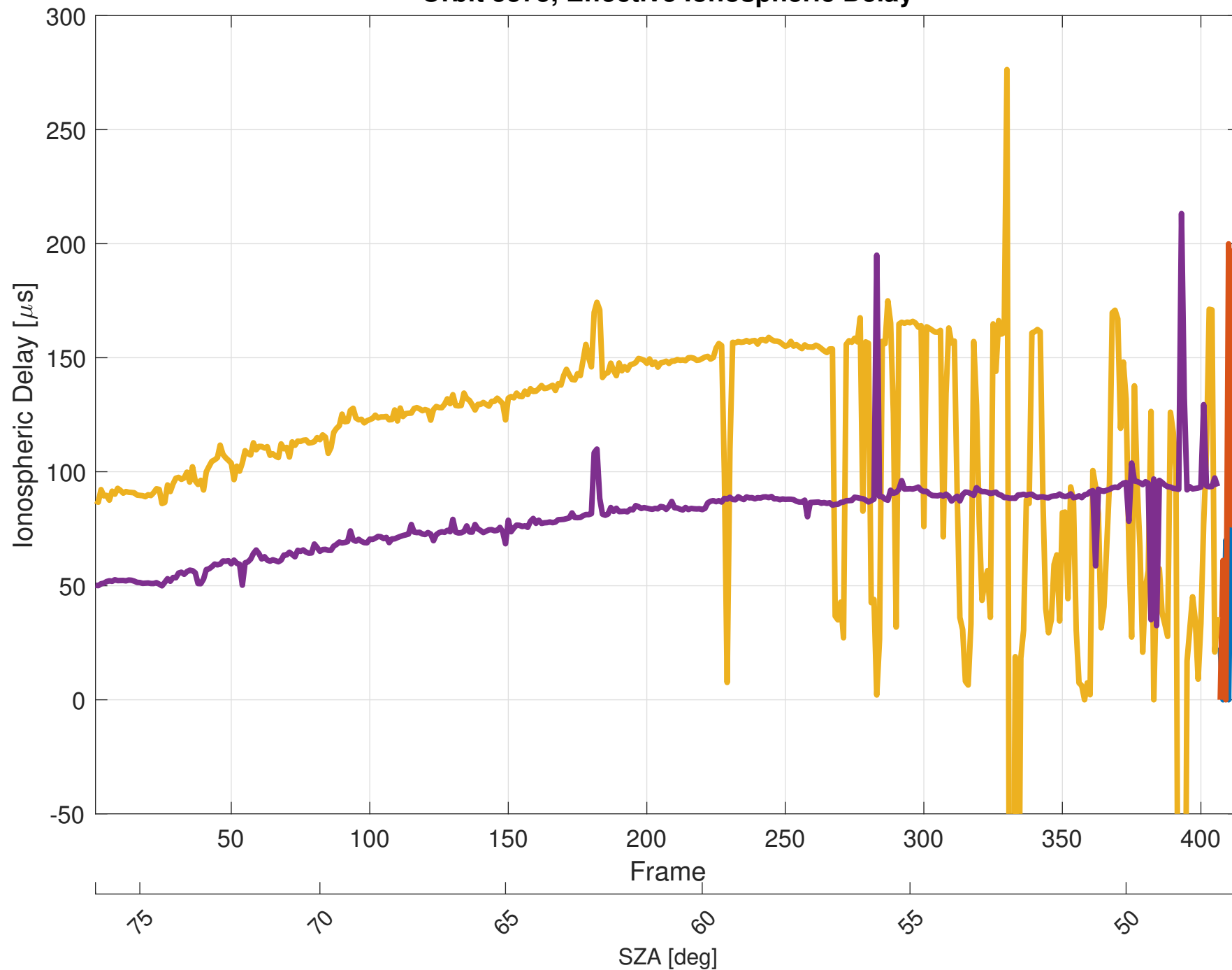
Orbit 5375, Effective Ionospheric Delay
