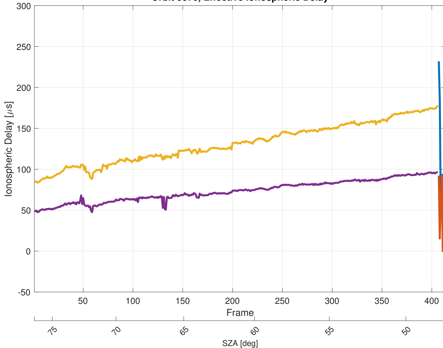
Orbit 5376, Effective Ionospheric Delay
