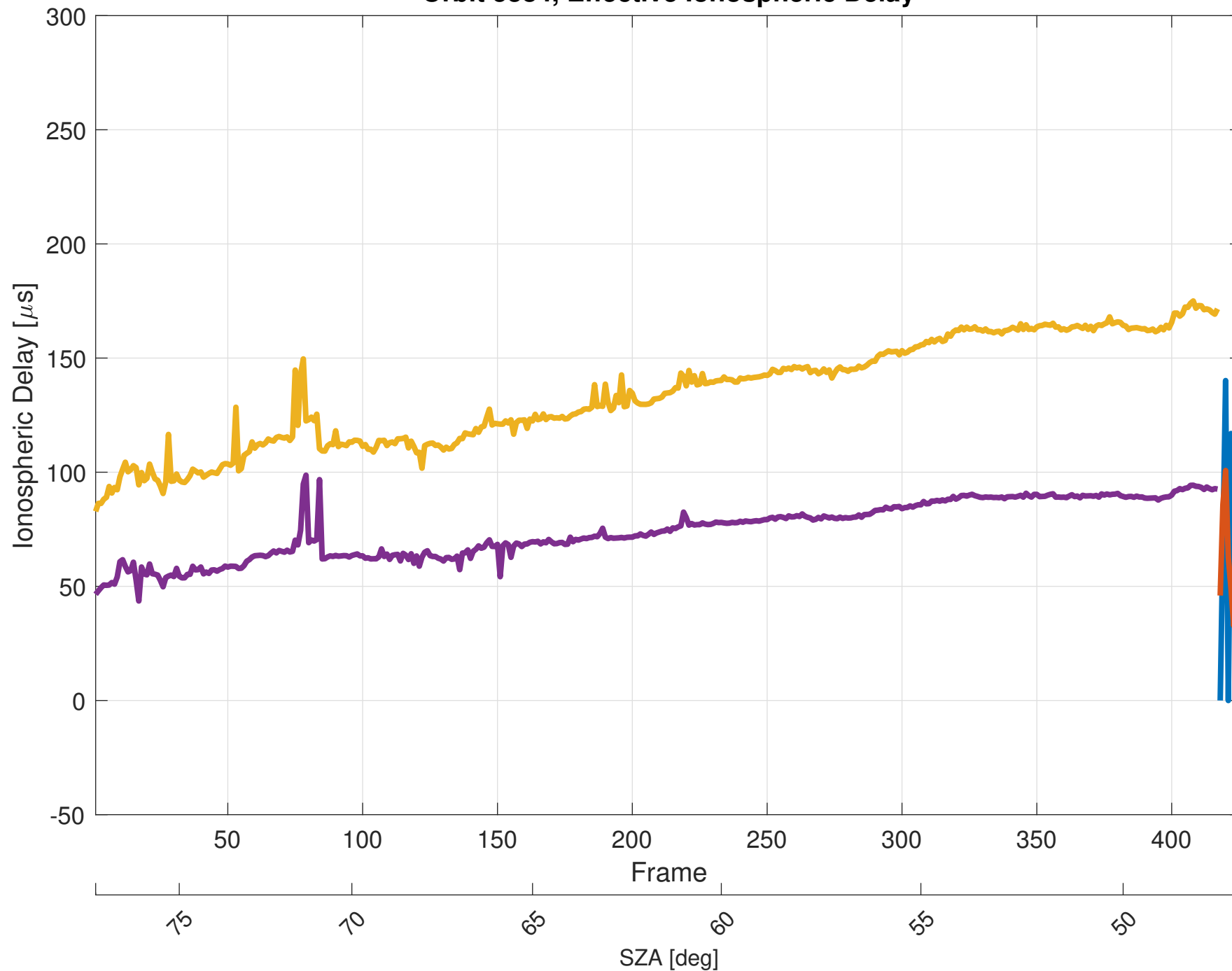
Orbit 5384, Effective Ionospheric Delay
