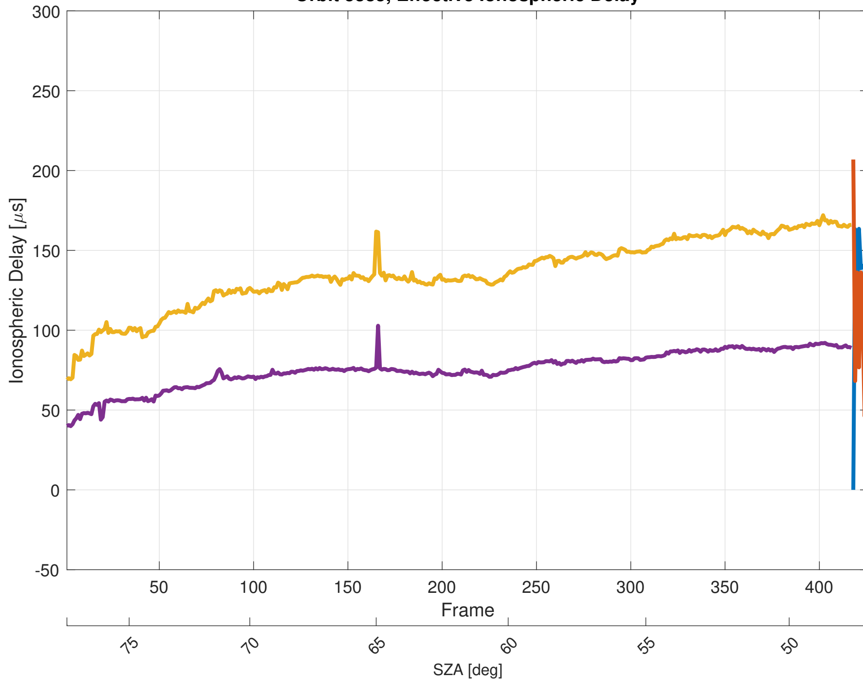
Orbit 5385, Effective Ionospheric Delay
