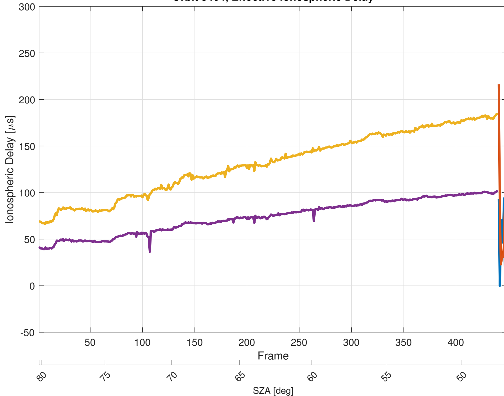
Orbit 5404, Effective Ionospheric Delay
