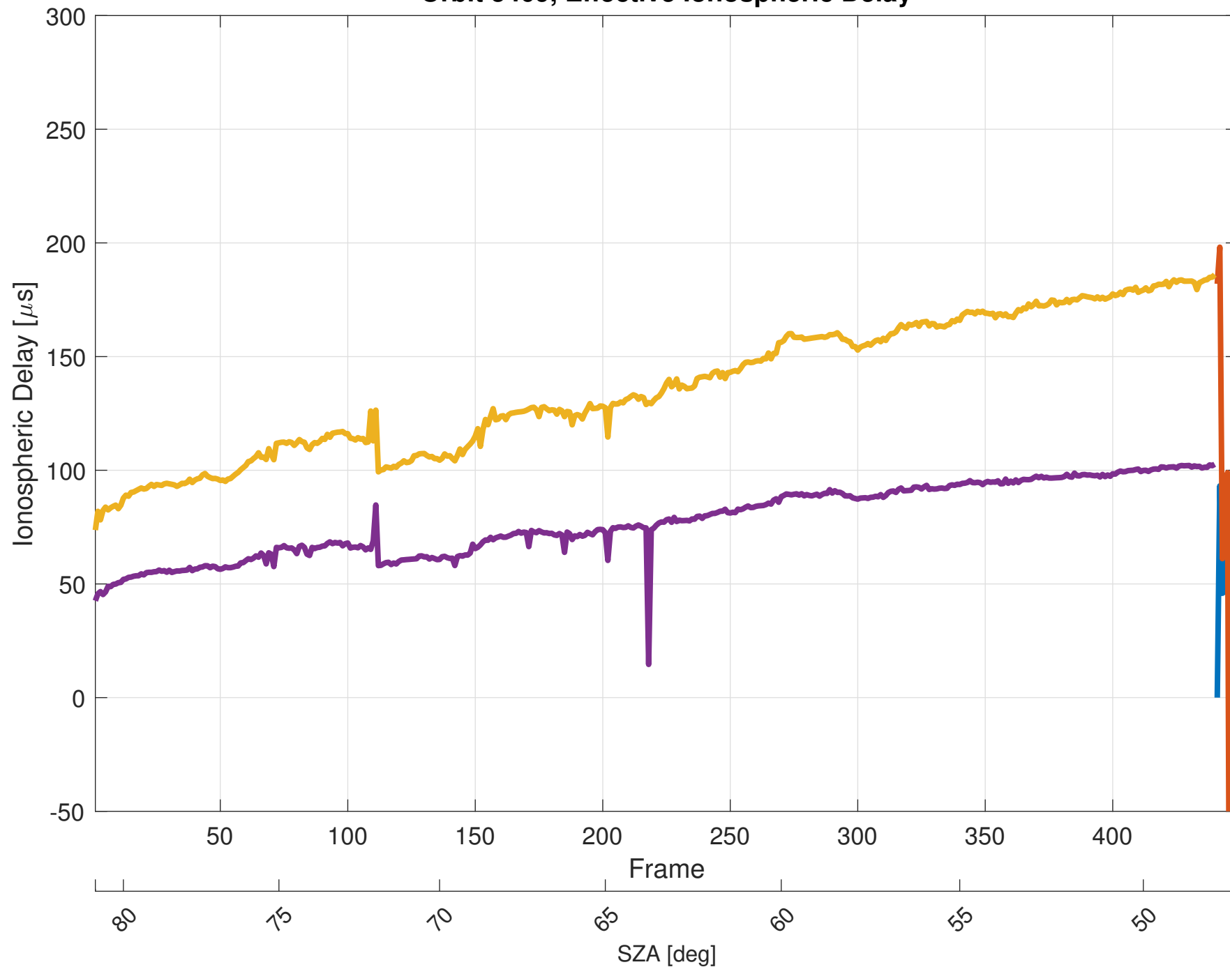
Orbit 5409, Effective Ionospheric Delay
