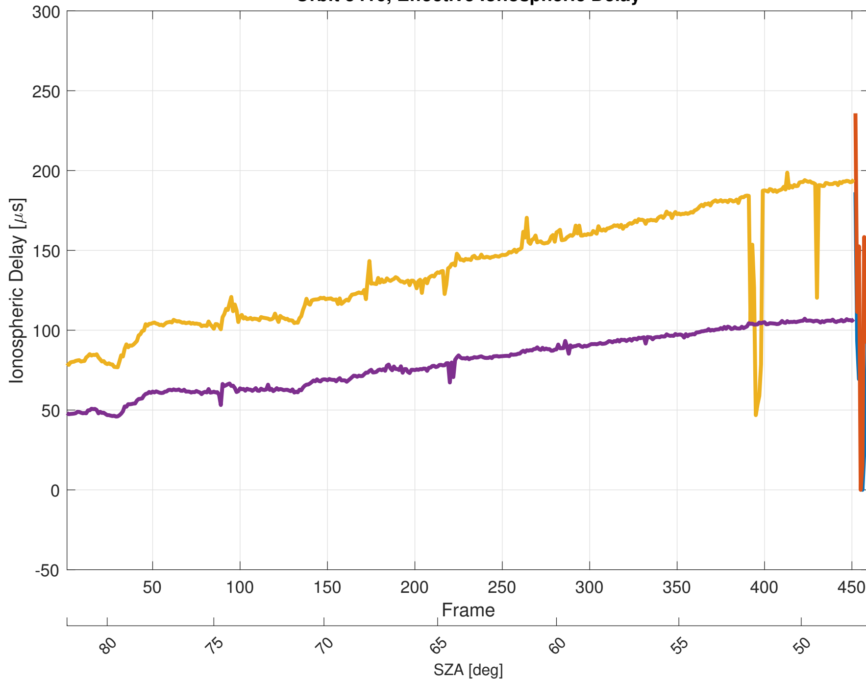
Orbit 5416, Effective Ionospheric Delay
