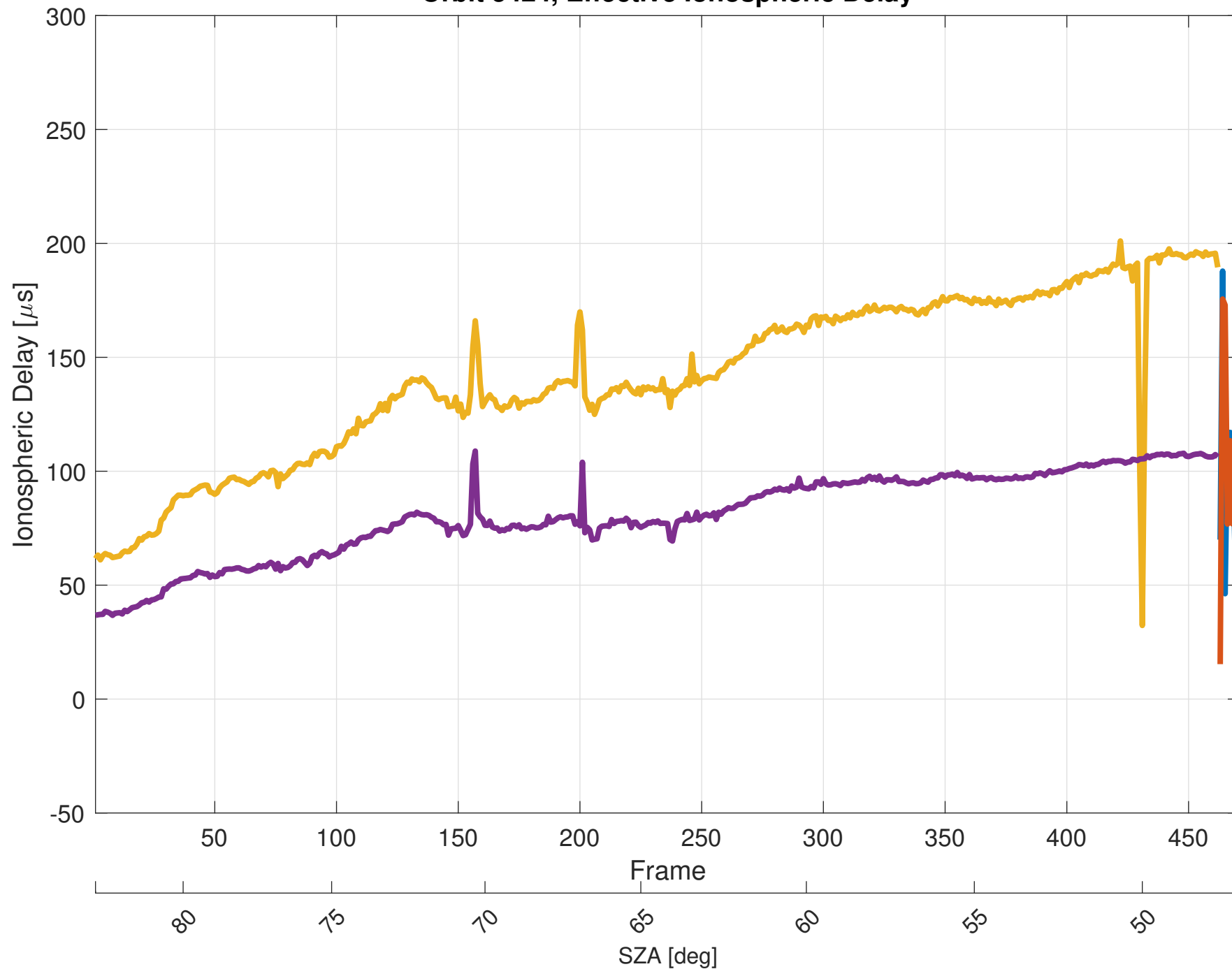
Orbit 5424, Effective Ionospheric Delay
