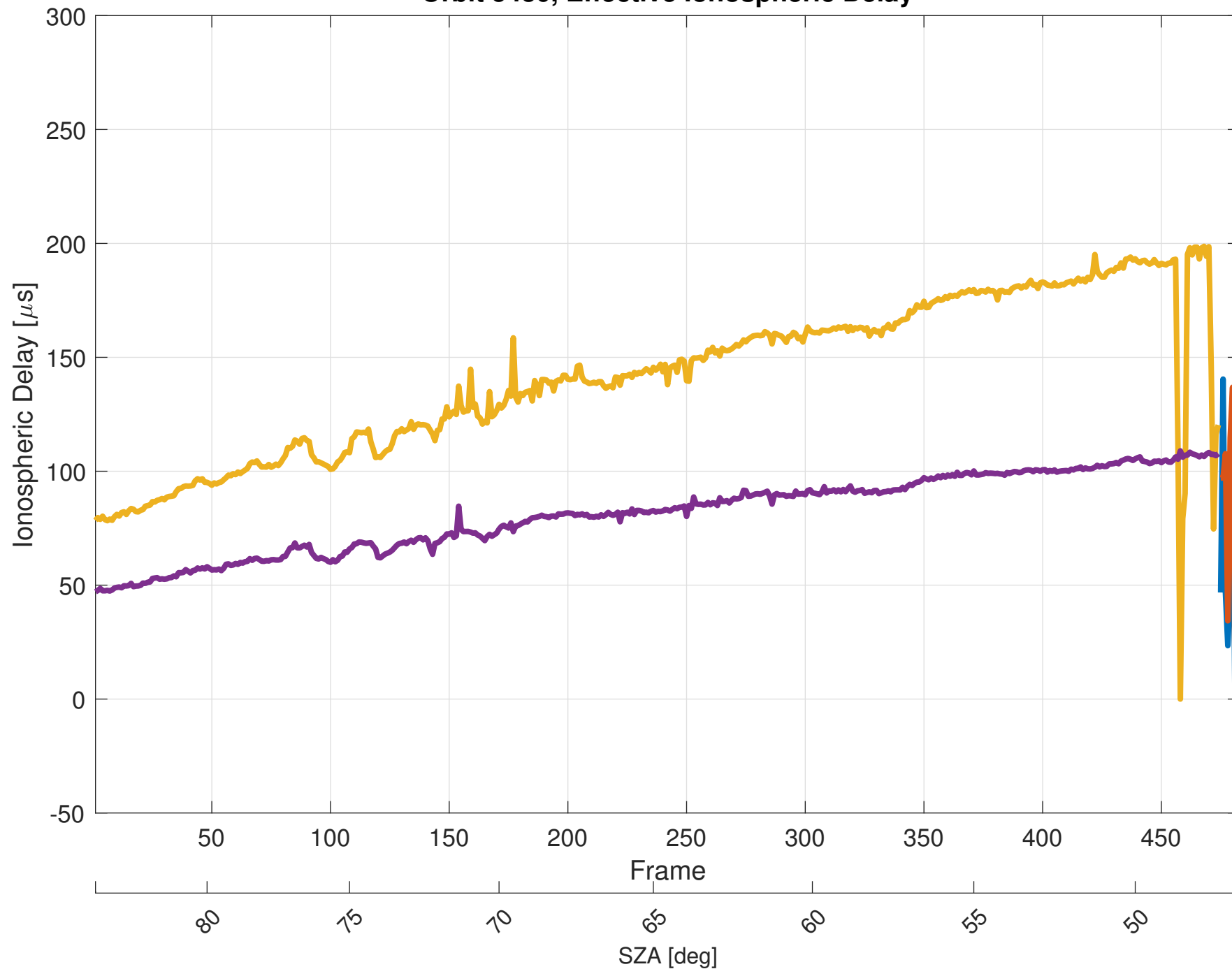
Orbit 5430, Effective Ionospheric Delay
