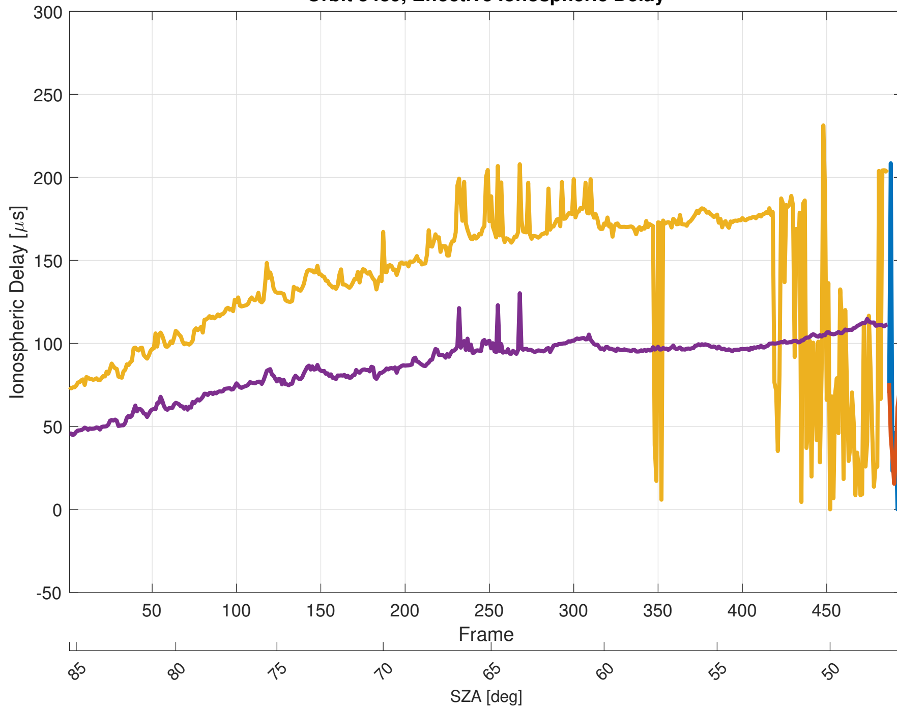
Orbit 5439, Effective Ionospheric Delay
