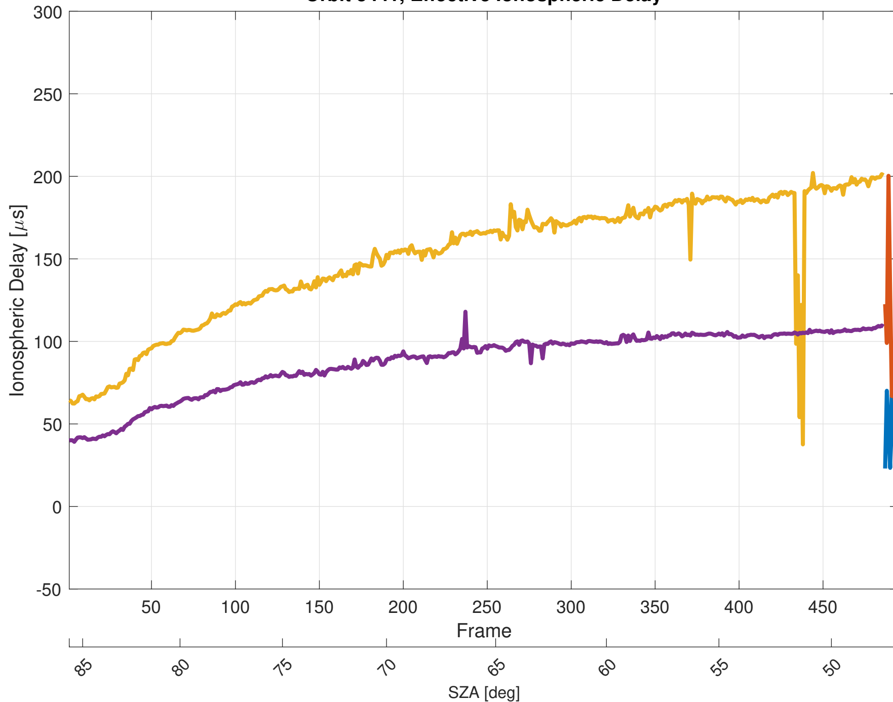
Orbit 5441, Effective Ionospheric Delay
