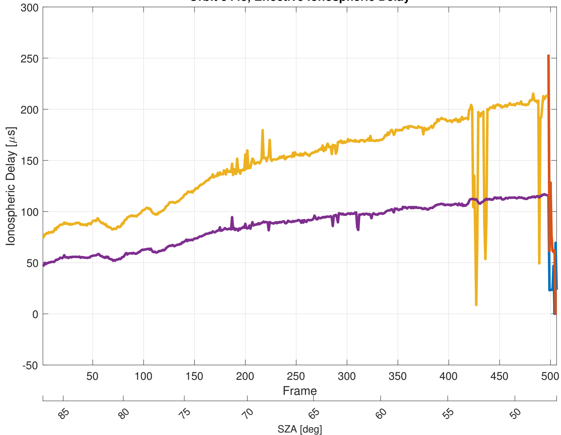
Orbit 5448, Effective Ionospheric Delay
