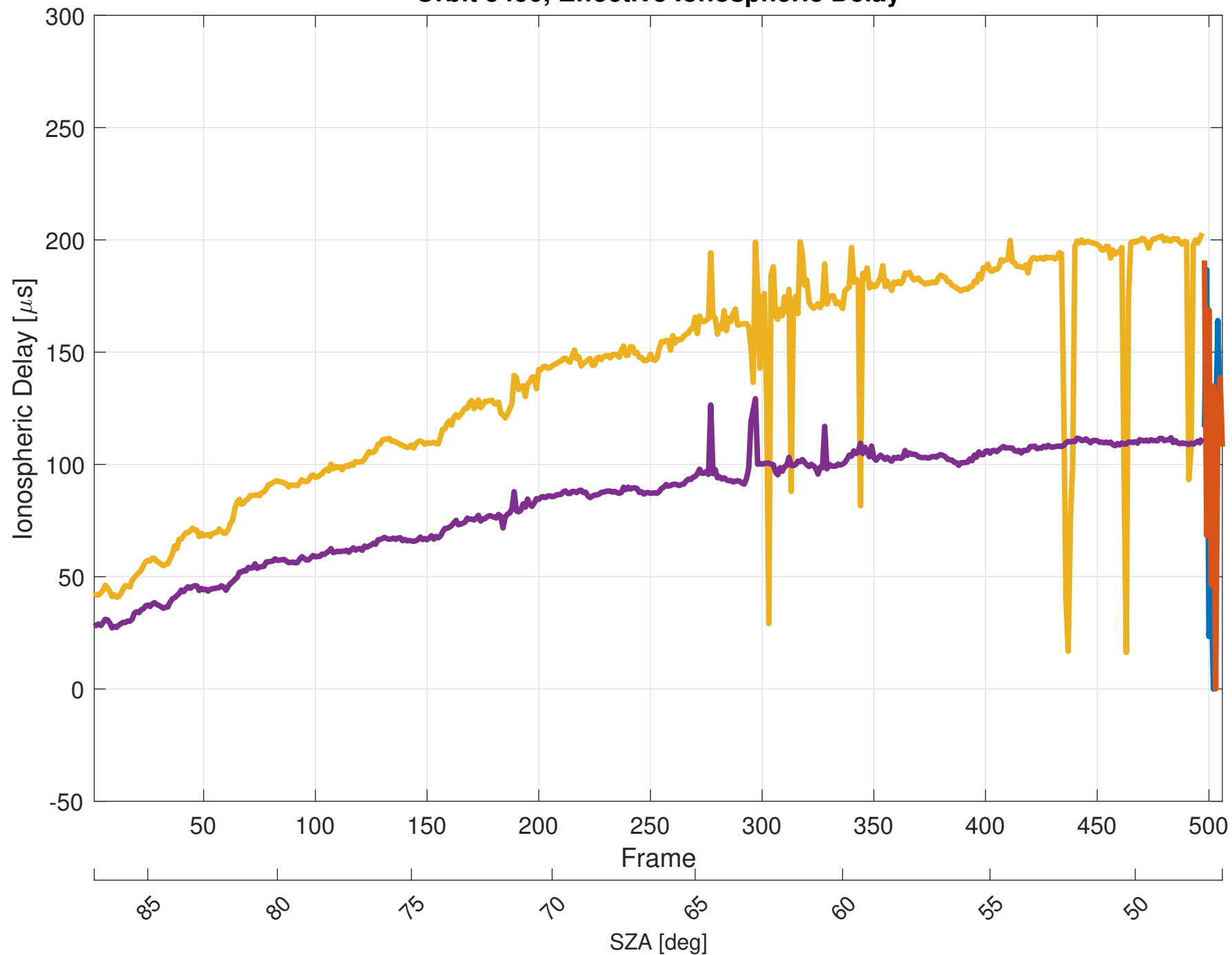
Orbit 5450, Effective Ionospheric Delay
