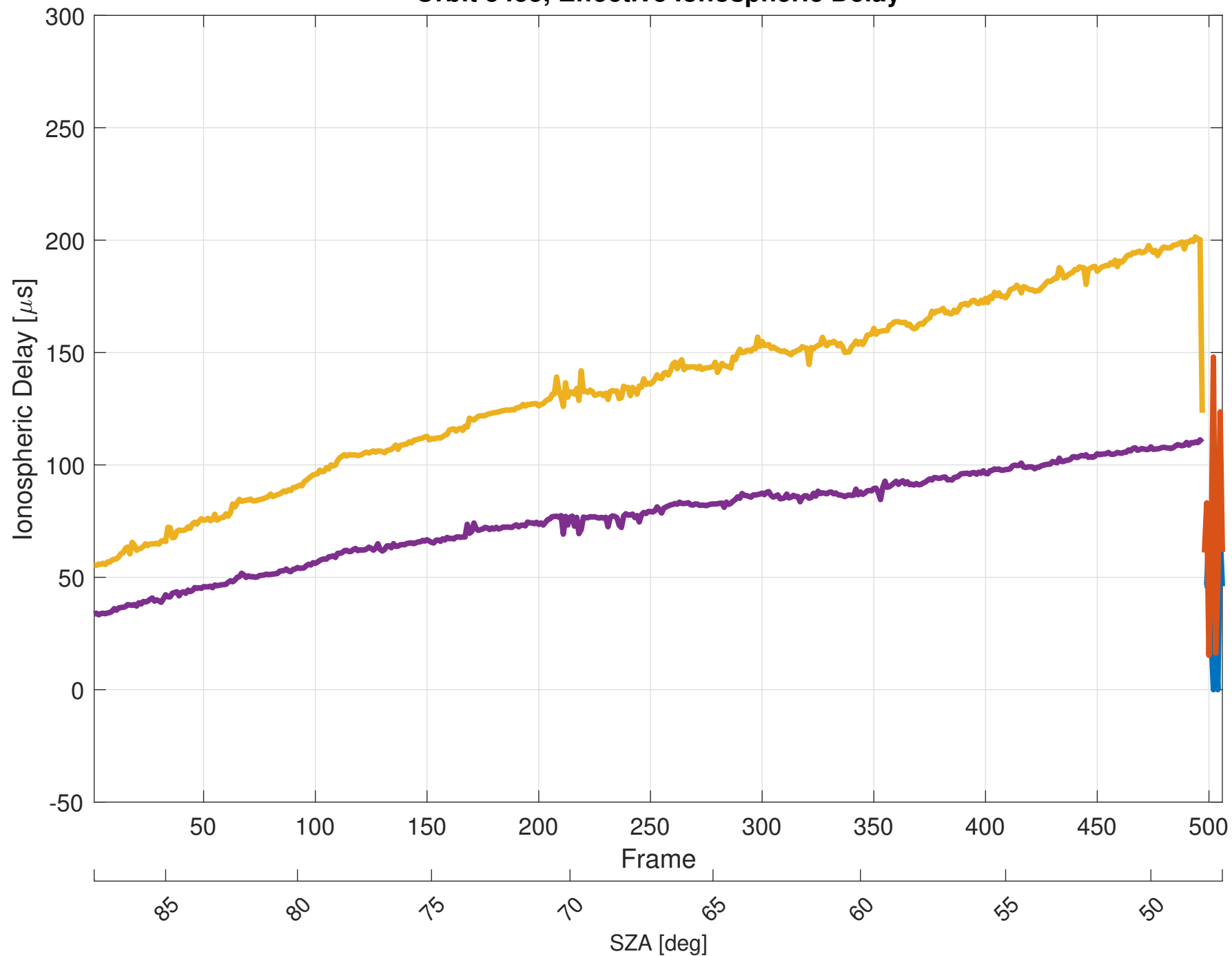
Orbit 5455, Effective Ionospheric Delay
