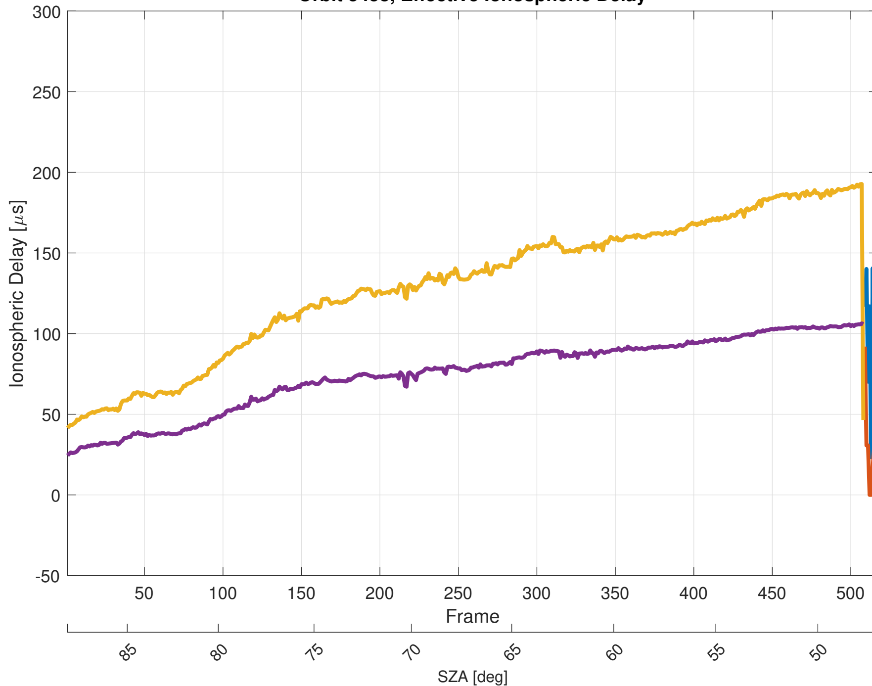
Orbit 5458, Effective Ionospheric Delay
