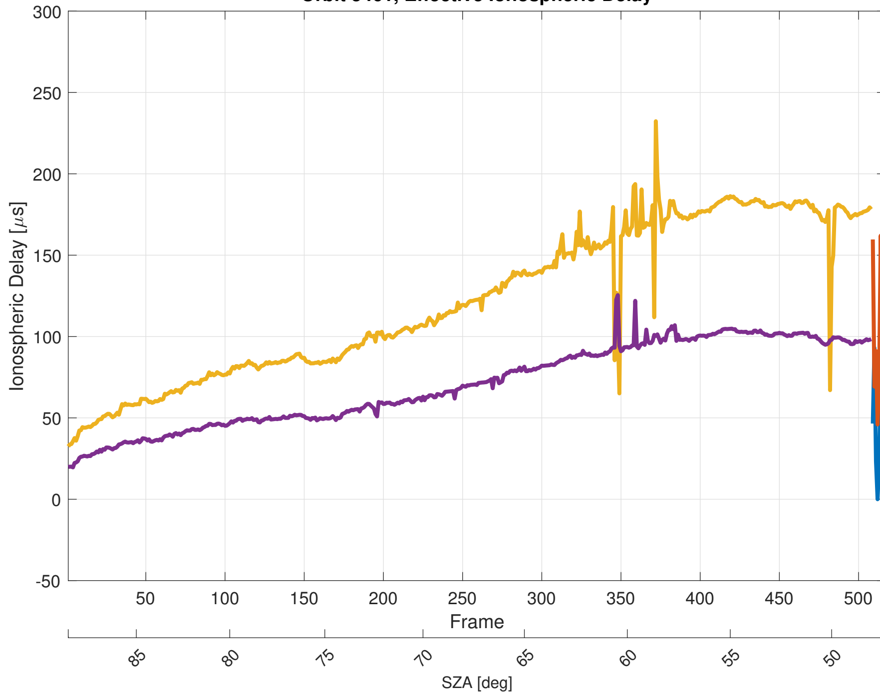
Orbit 5461, Effective Ionospheric Delay
