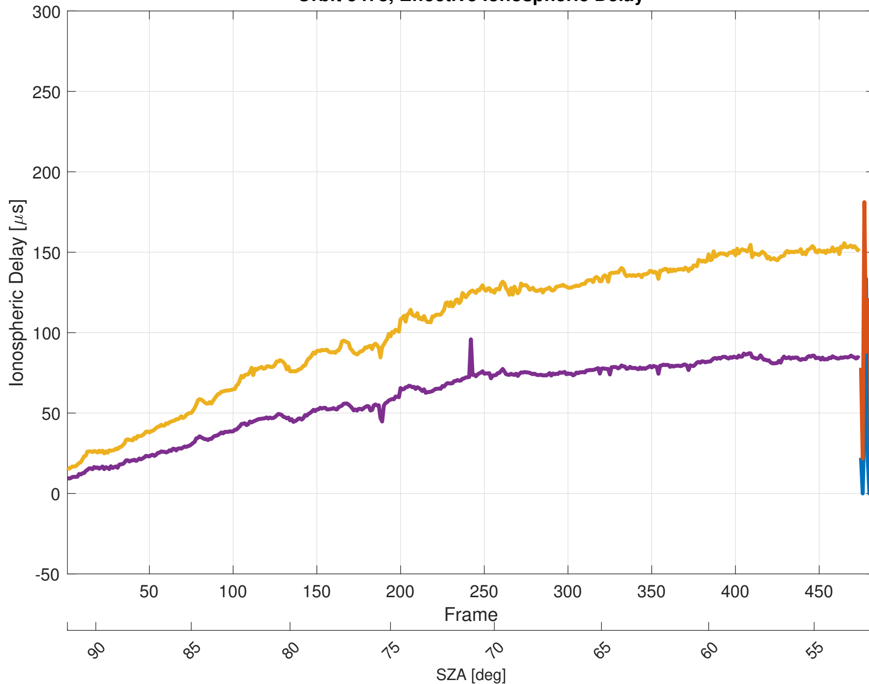
Orbit 5478, Effective Ionospheric Delay
