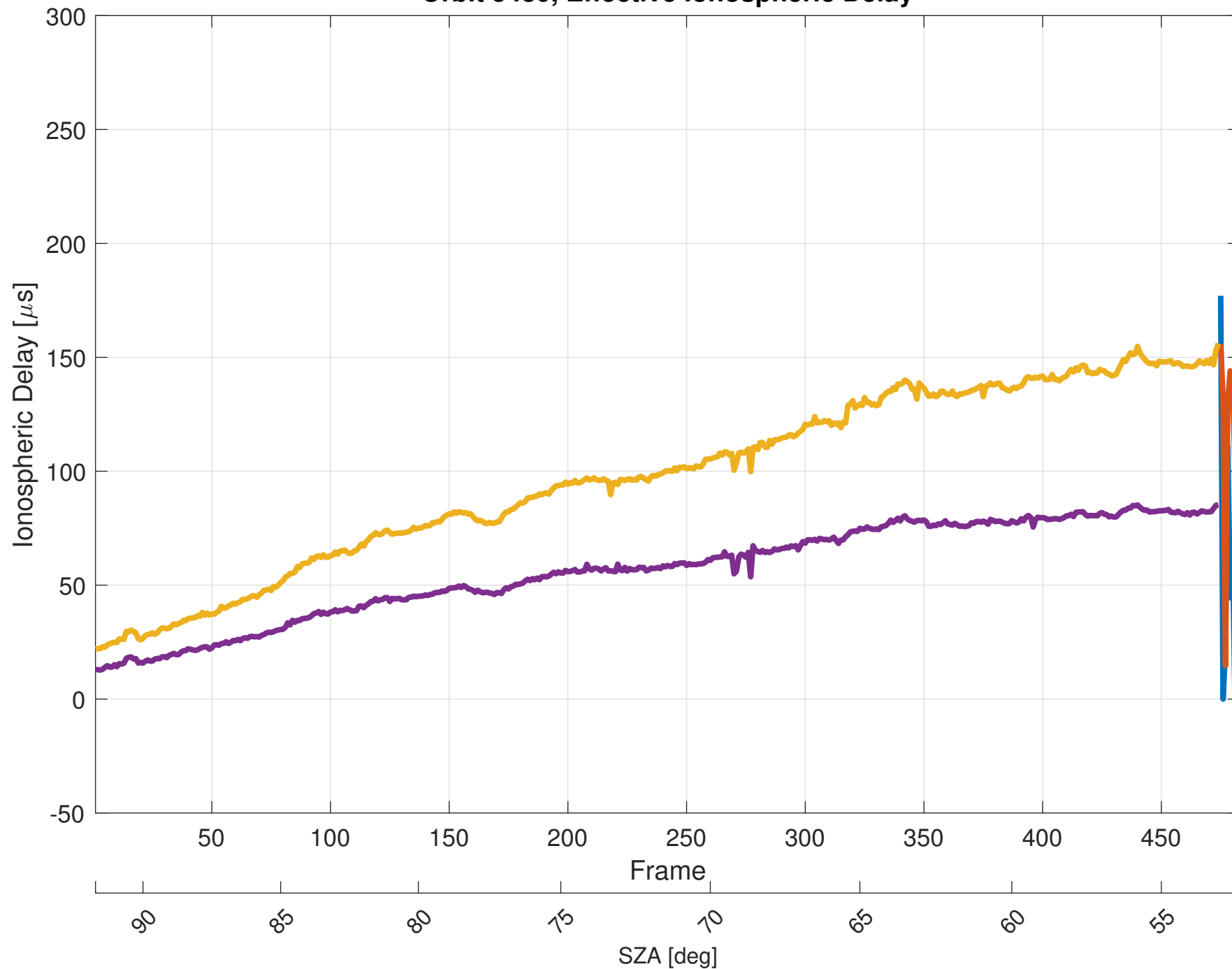
Orbit 5480, Effective Ionospheric Delay
