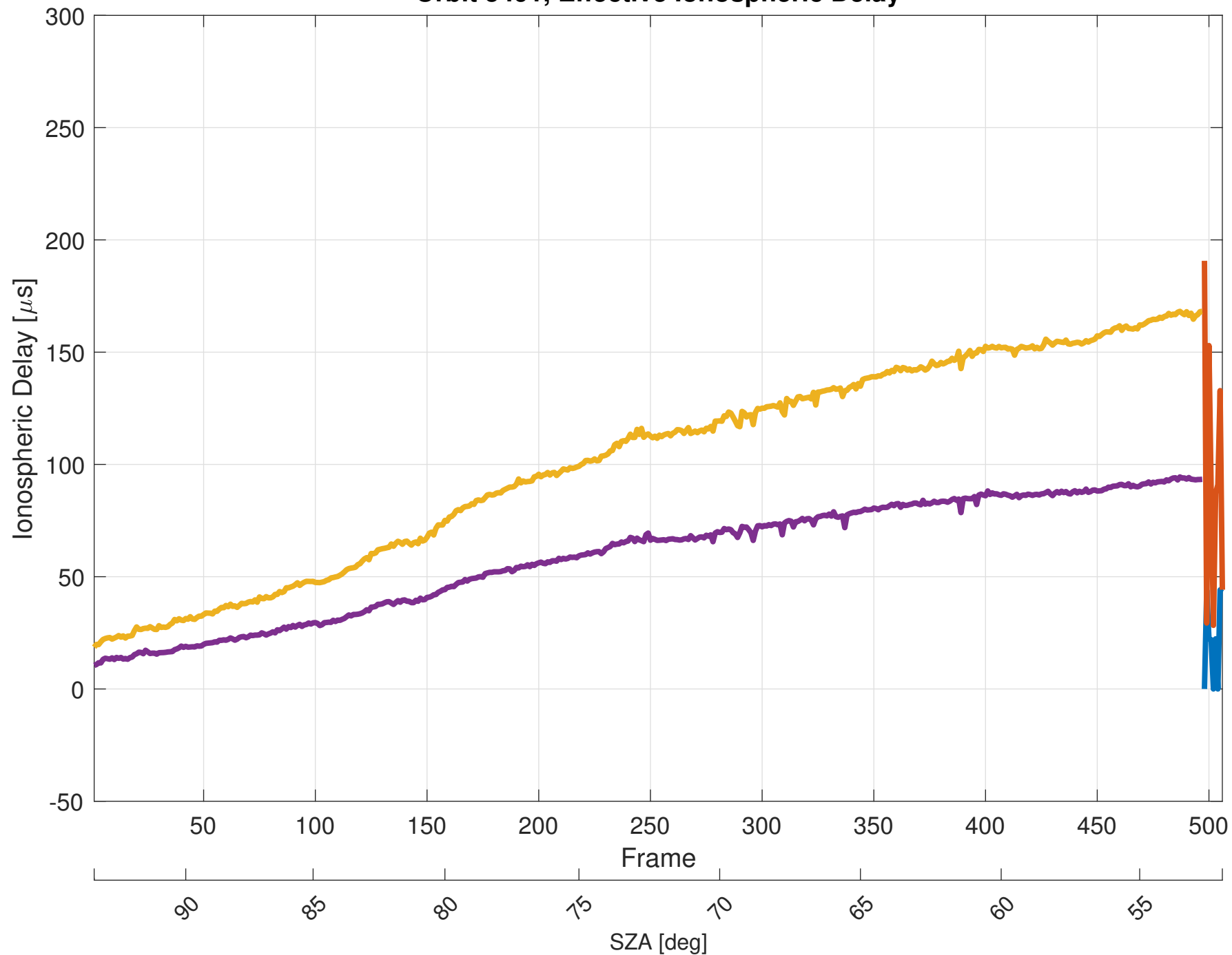
Orbit 5491, Effective Ionospheric Delay
