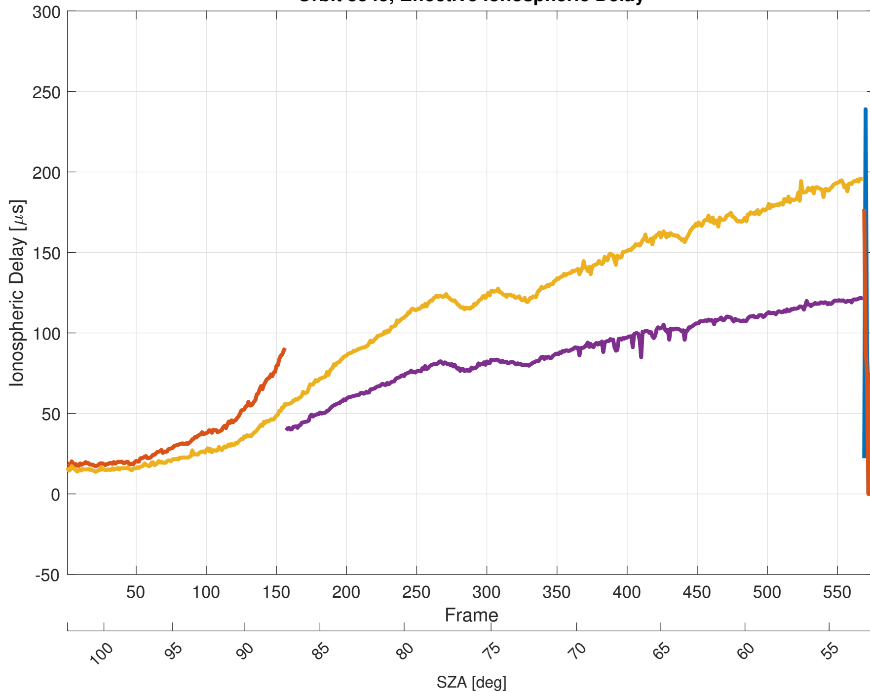
Orbit 5545, Effective Ionospheric Delay
