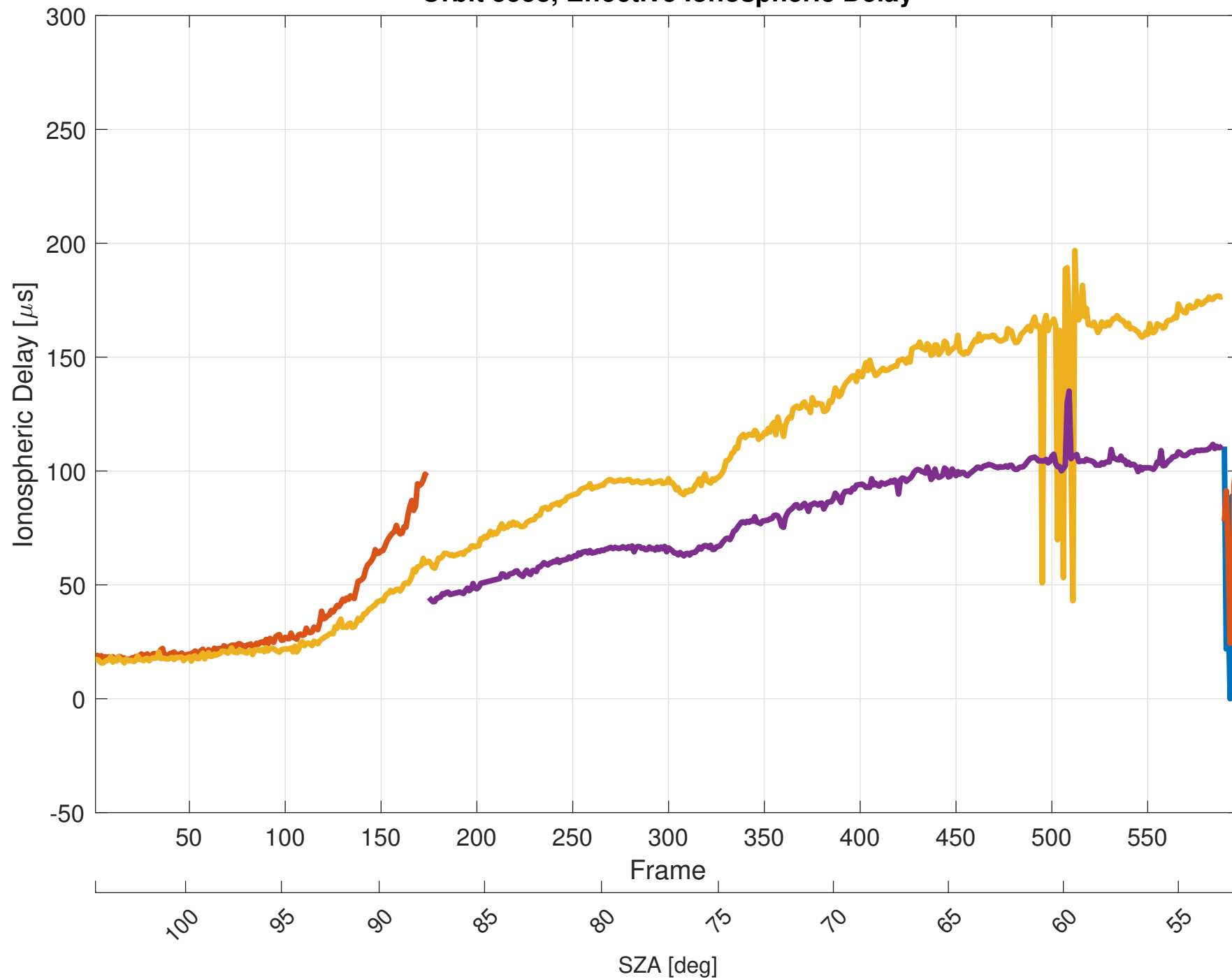
Orbit 5558, Effective Ionospheric Delay
