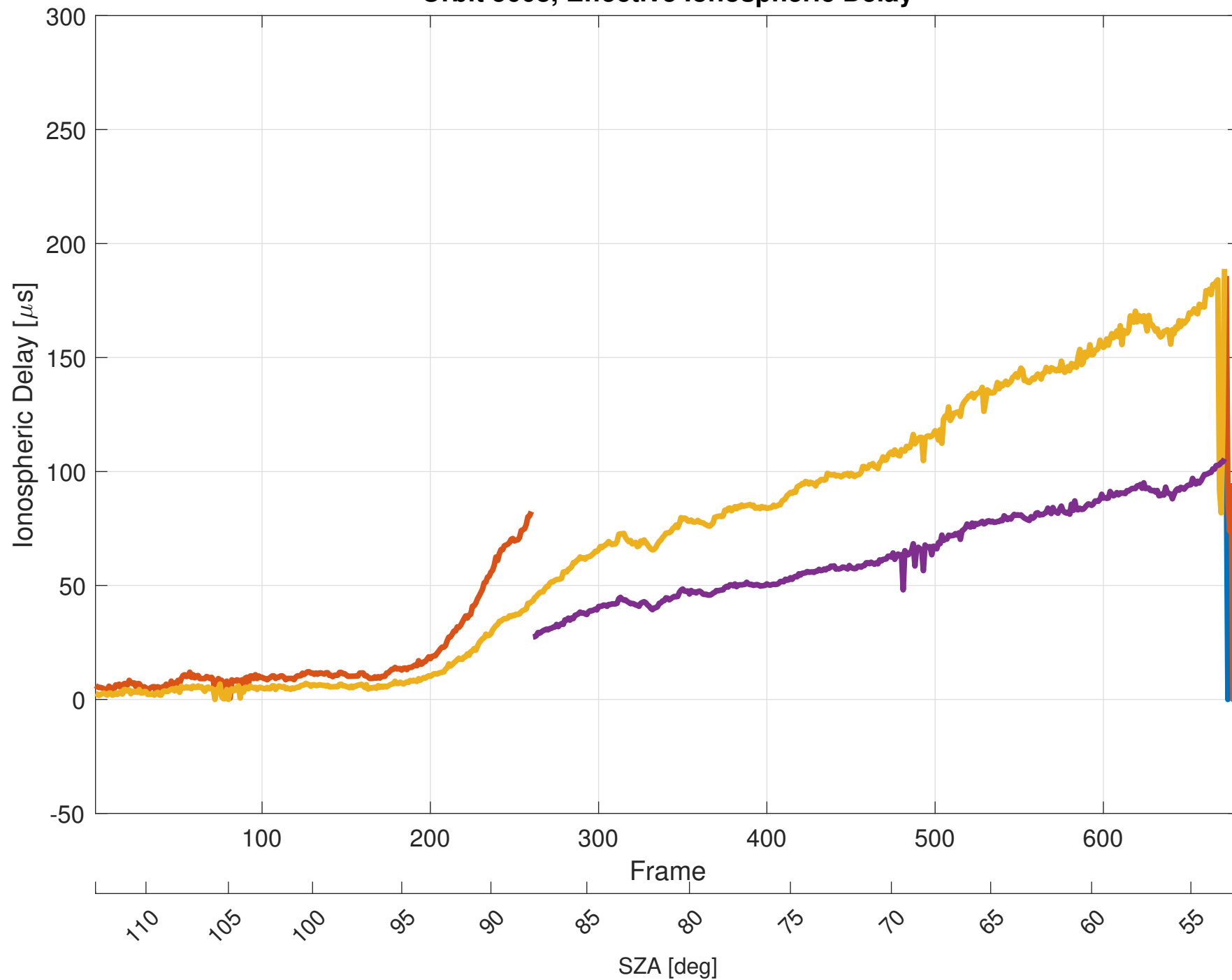
Orbit 5608, Effective Ionospheric Delay
