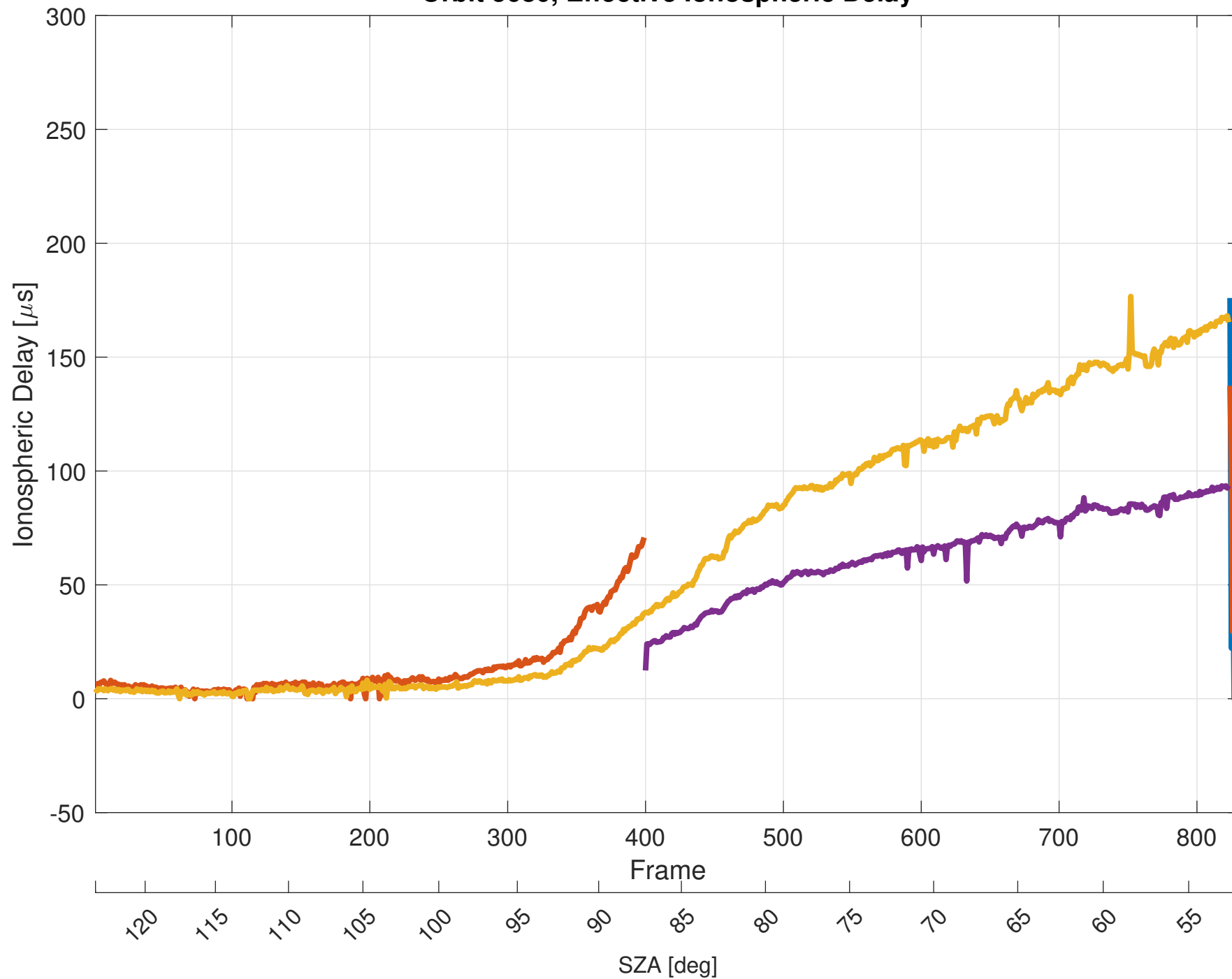
Orbit 5680, Effective Ionospheric Delay
