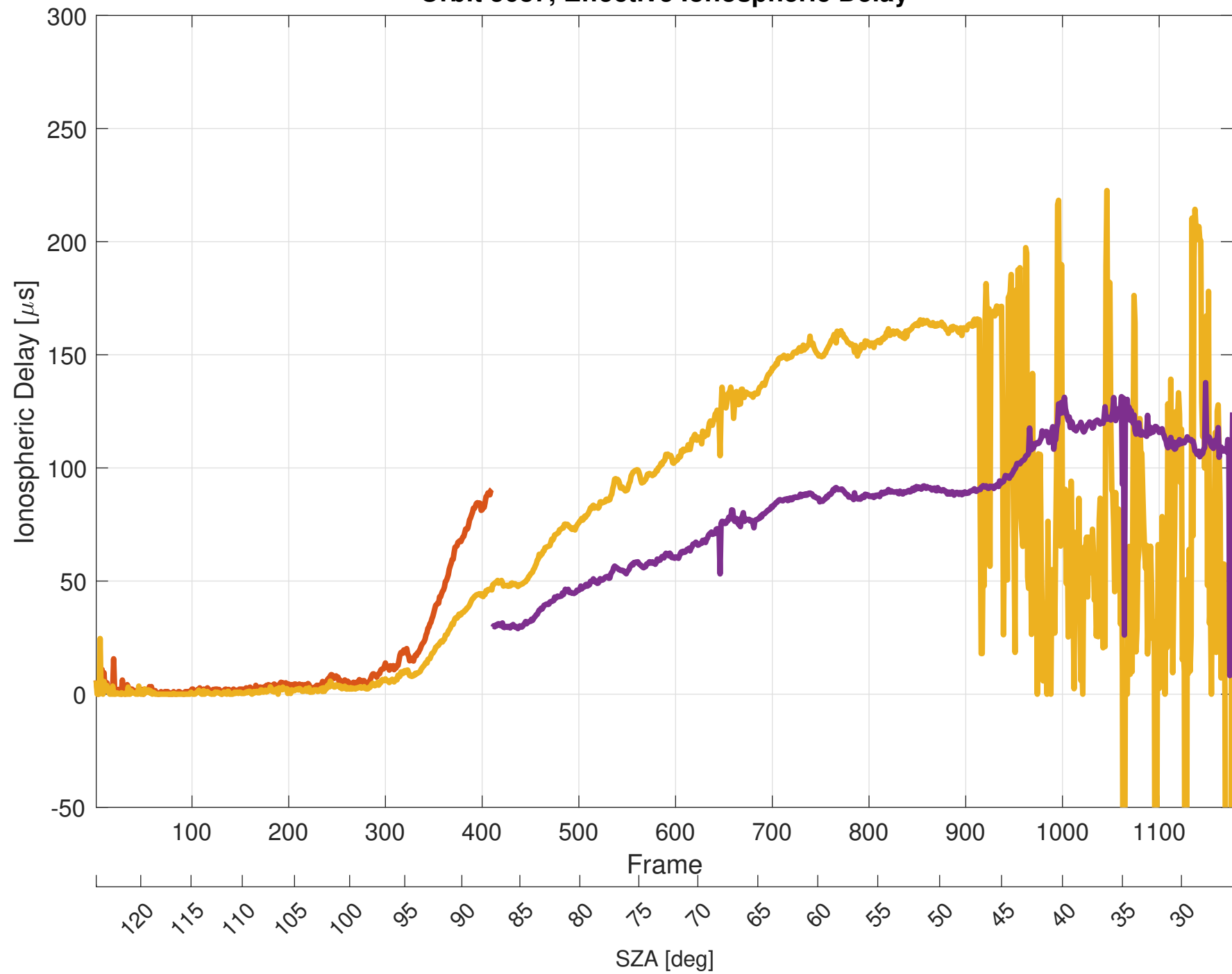
Orbit 5687, Effective Ionospheric Delay
