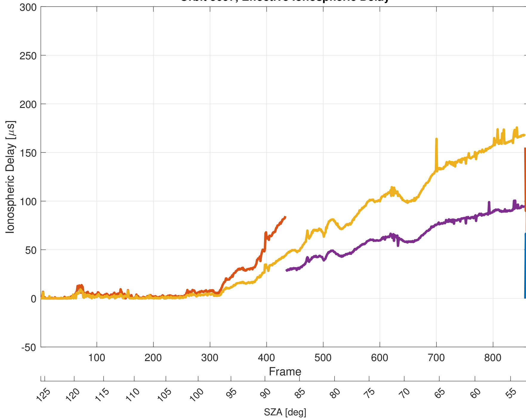
Orbit 5697, Effective Ionospheric Delay
