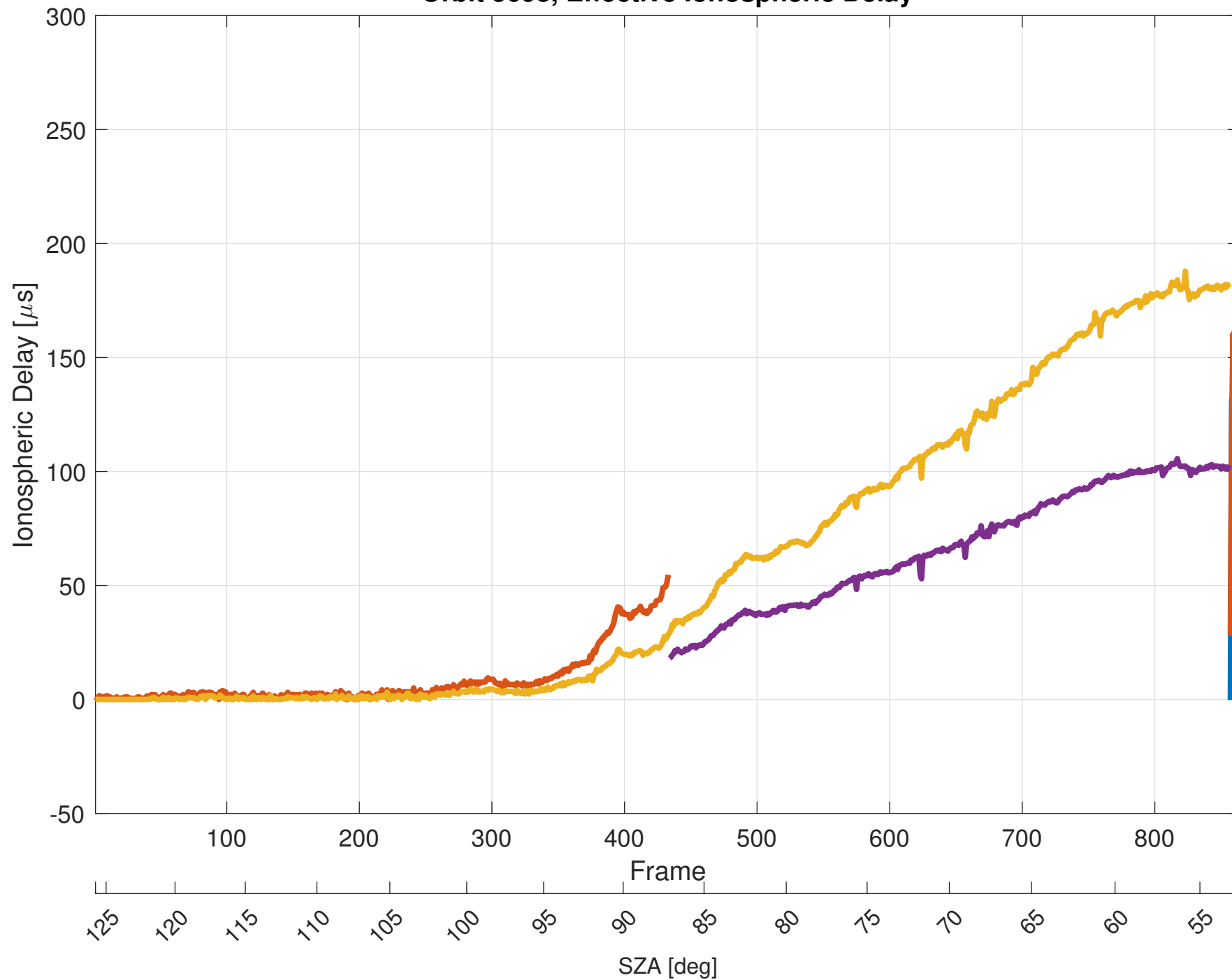
Orbit 5698, Effective Ionospheric Delay
