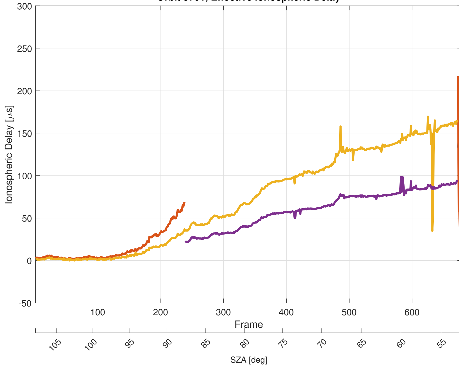
Orbit 5701, Effective Ionospheric Delay
