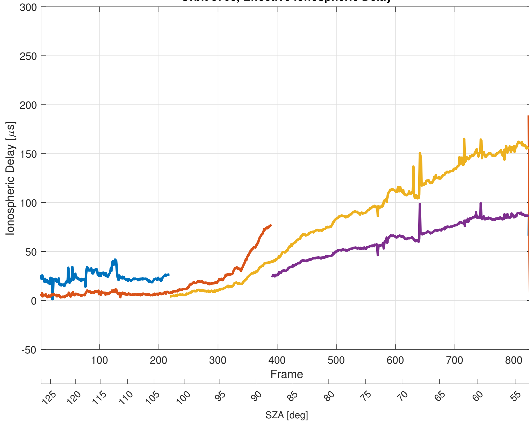
Orbit 5708, Effective Ionospheric Delay
