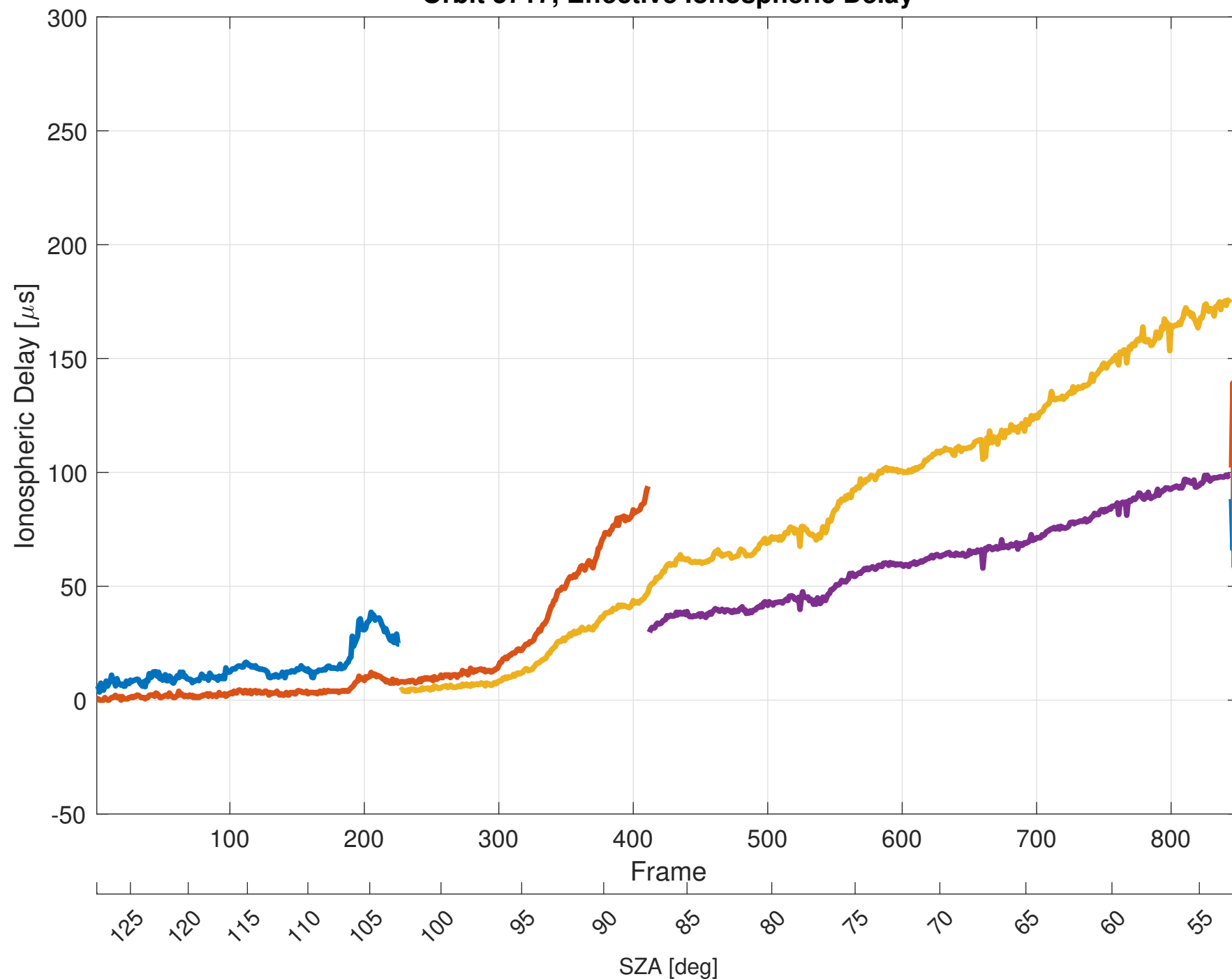
Orbit 5717, Effective Ionospheric Delay
