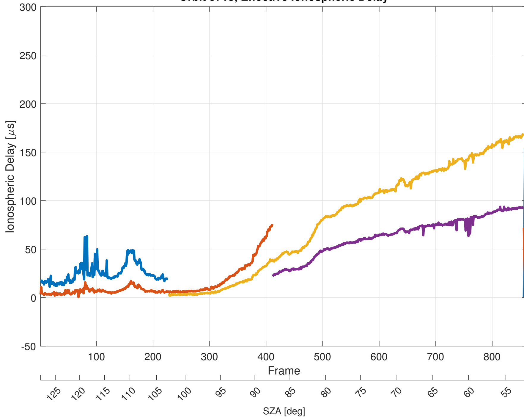
Orbit 5718, Effective Ionospheric Delay
