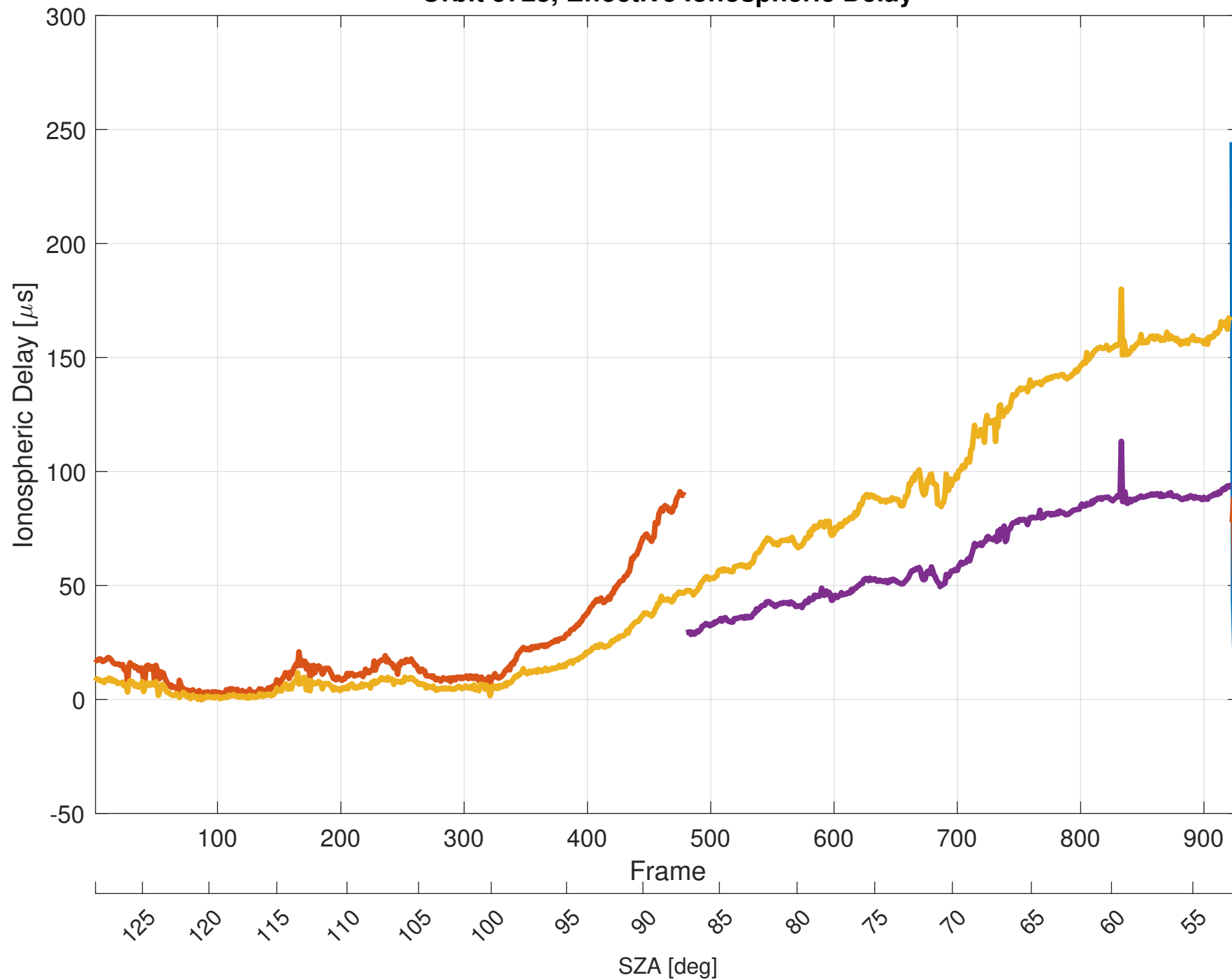
Orbit 5723, Effective Ionospheric Delay
