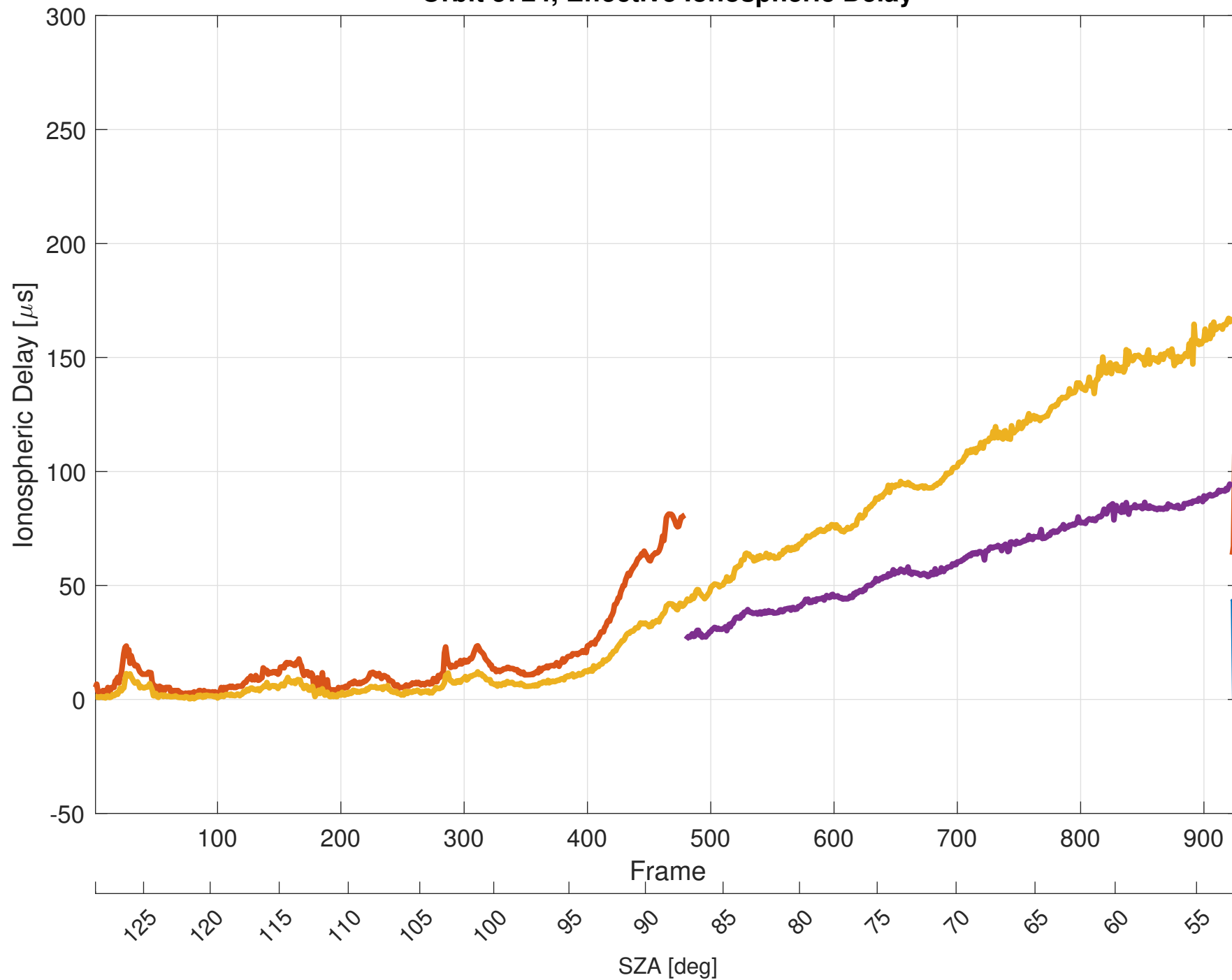
Orbit 5724, Effective Ionospheric Delay
