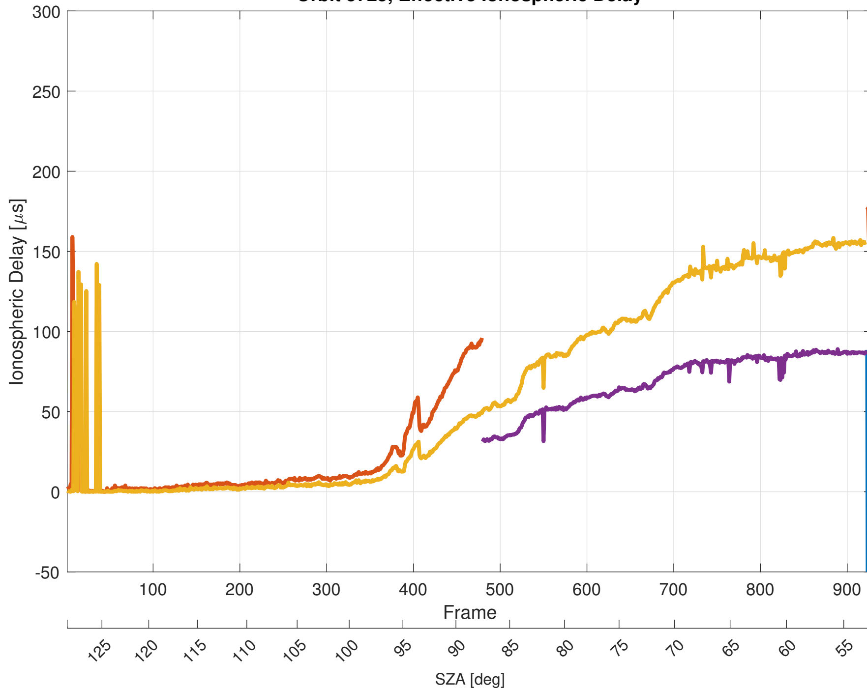
Orbit 5725, Effective Ionospheric Delay
