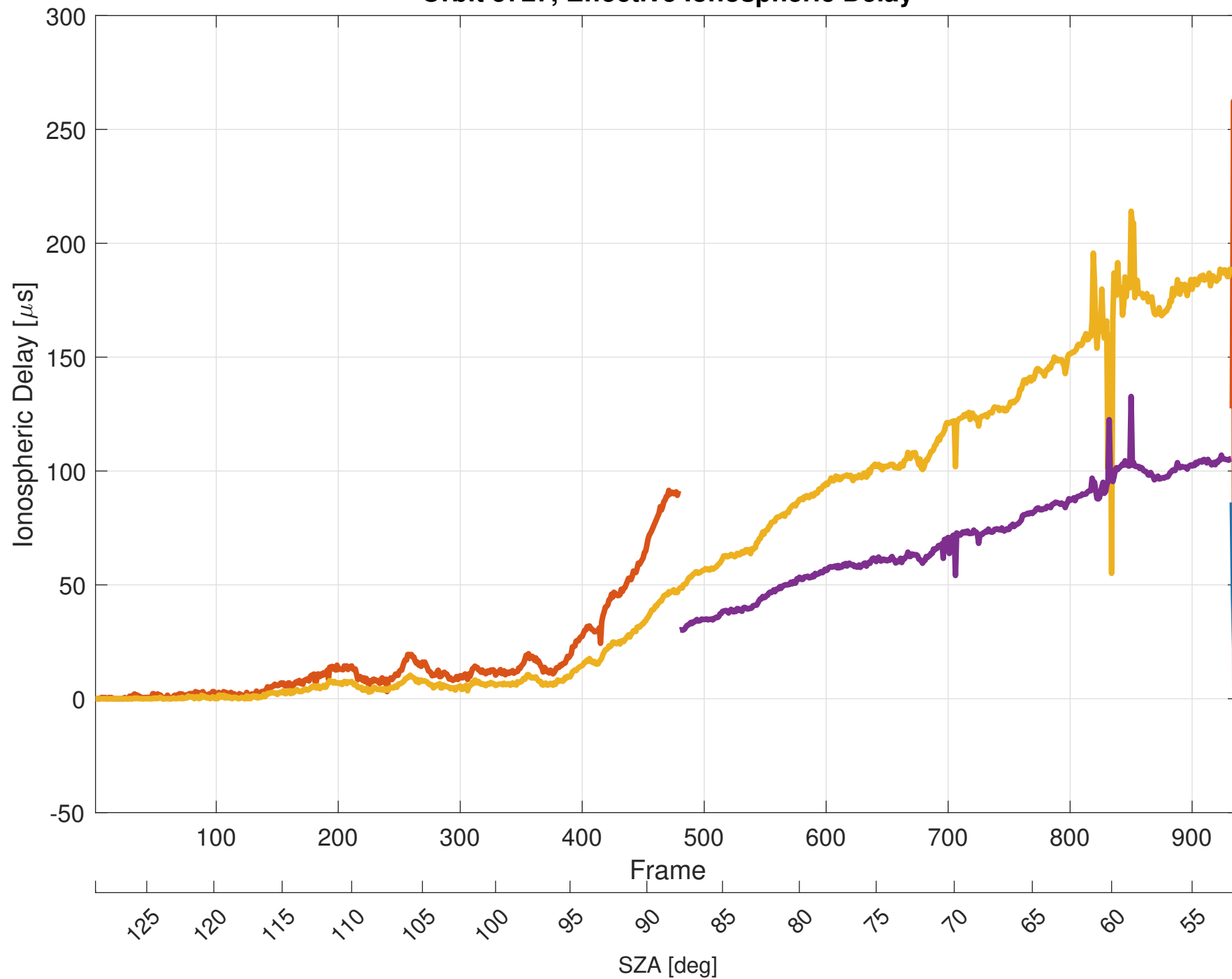
Orbit 5727, Effective Ionospheric Delay
