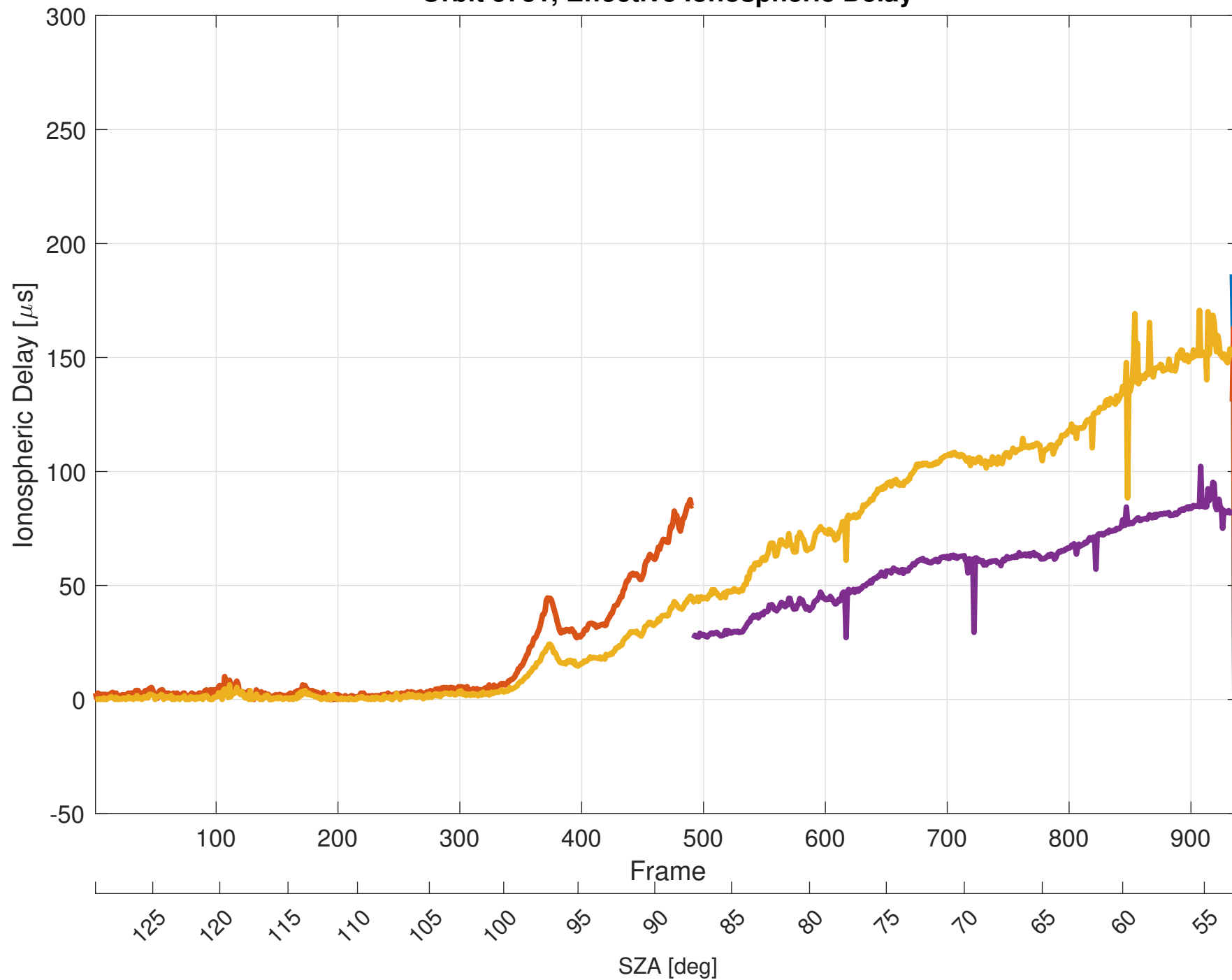
Orbit 5731, Effective Ionospheric Delay
