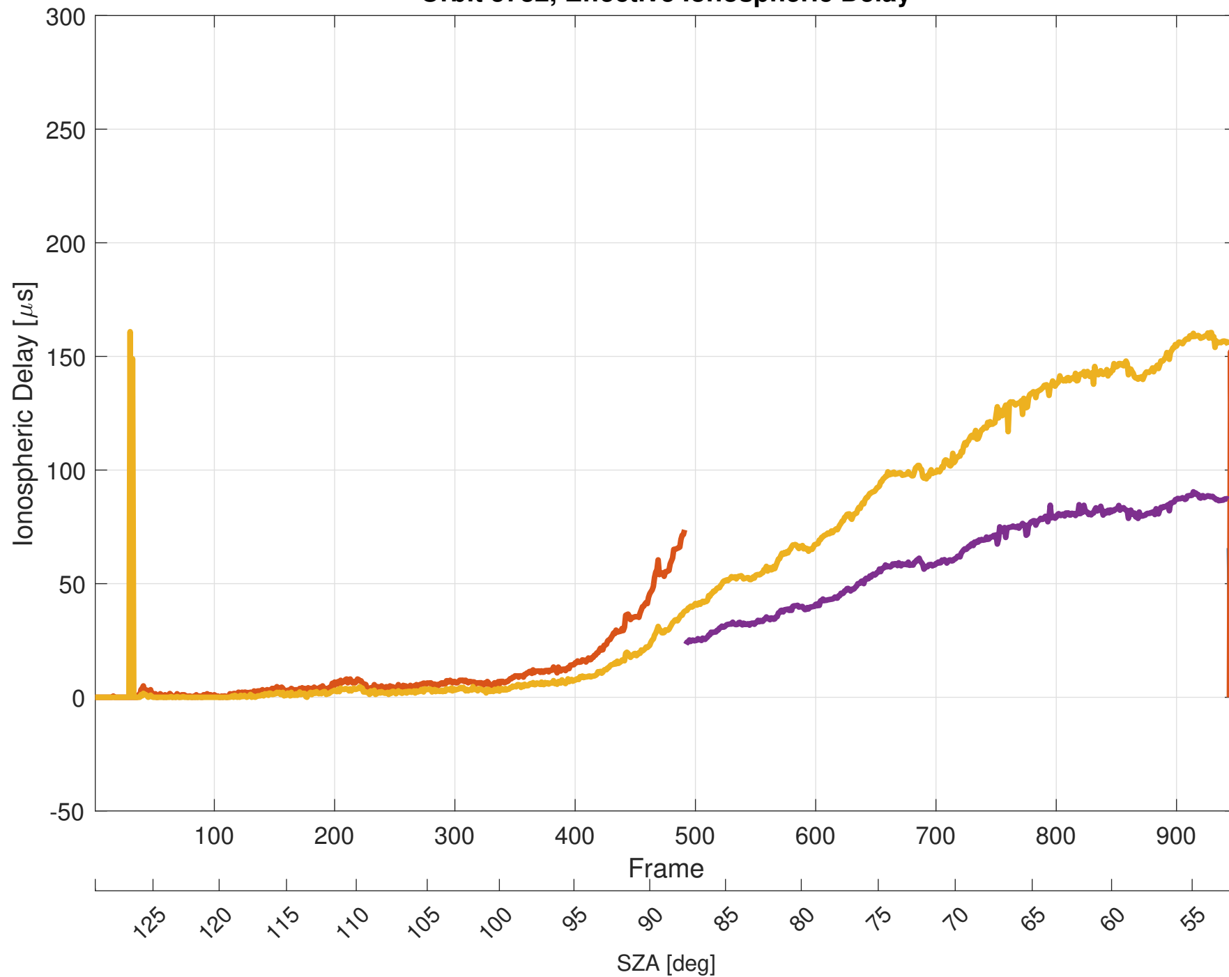
Orbit 5732, Effective Ionospheric Delay
